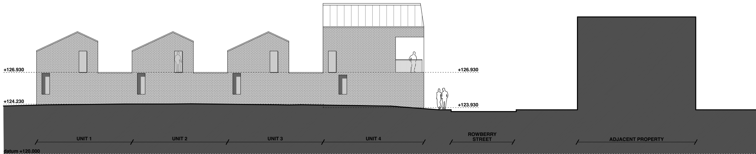
SCHALLENGE WALK ELEVATION (ONE)
