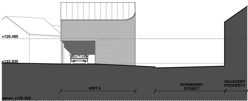
ELEVATION FIVE
