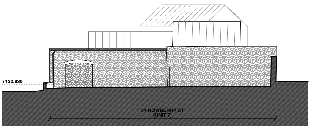
ELEVATION SIX
