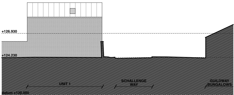
ELEVATION FOUR
