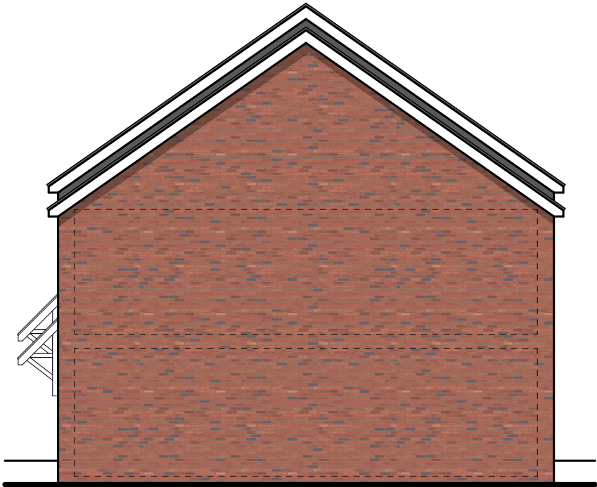
Plot 24 Side Elevation
