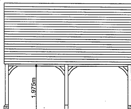
FRONT ELEVATION
