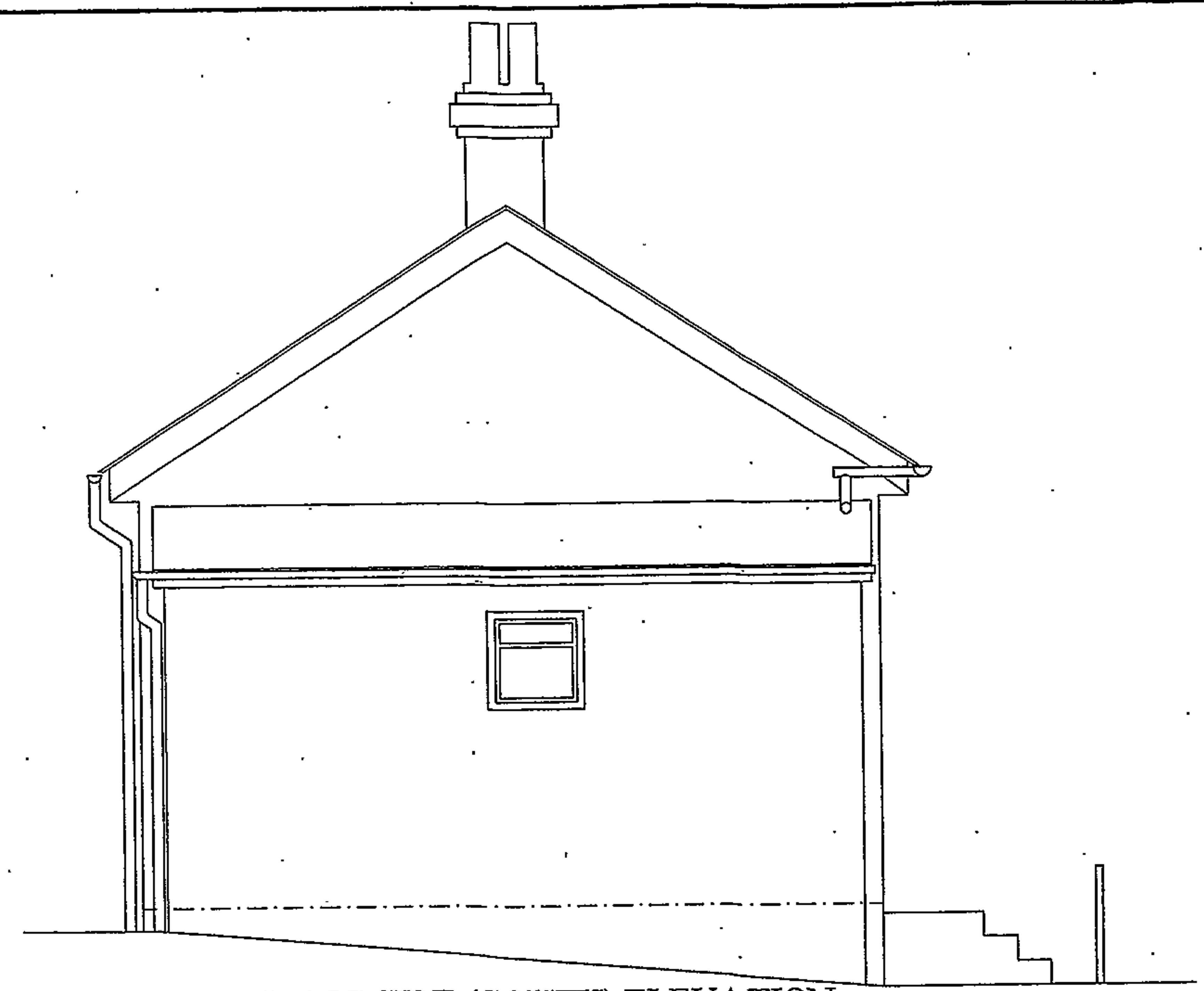
EXISTING SIDE (SOUTH) ELEVATION.
