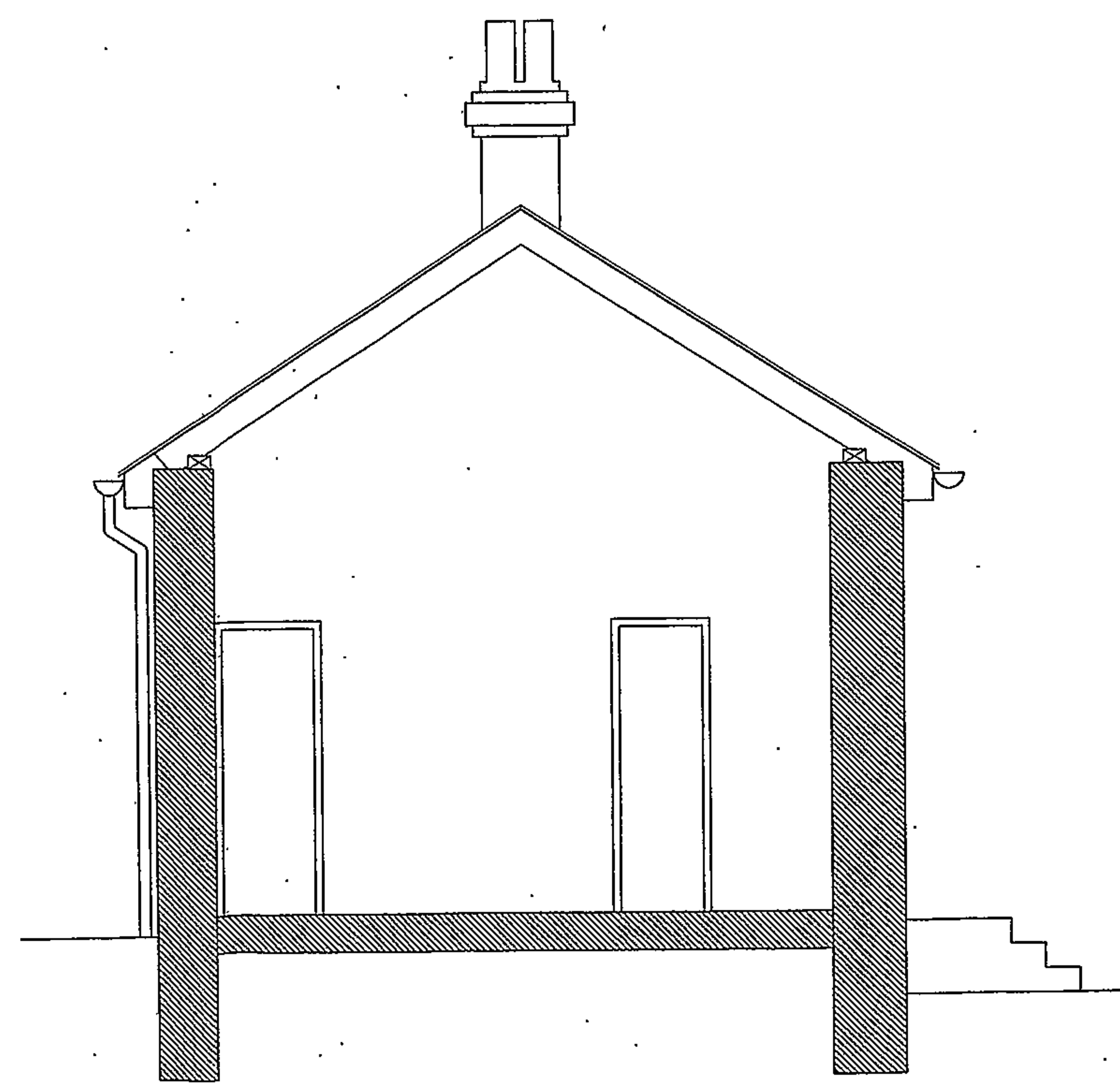
EXISTING SECTION.
