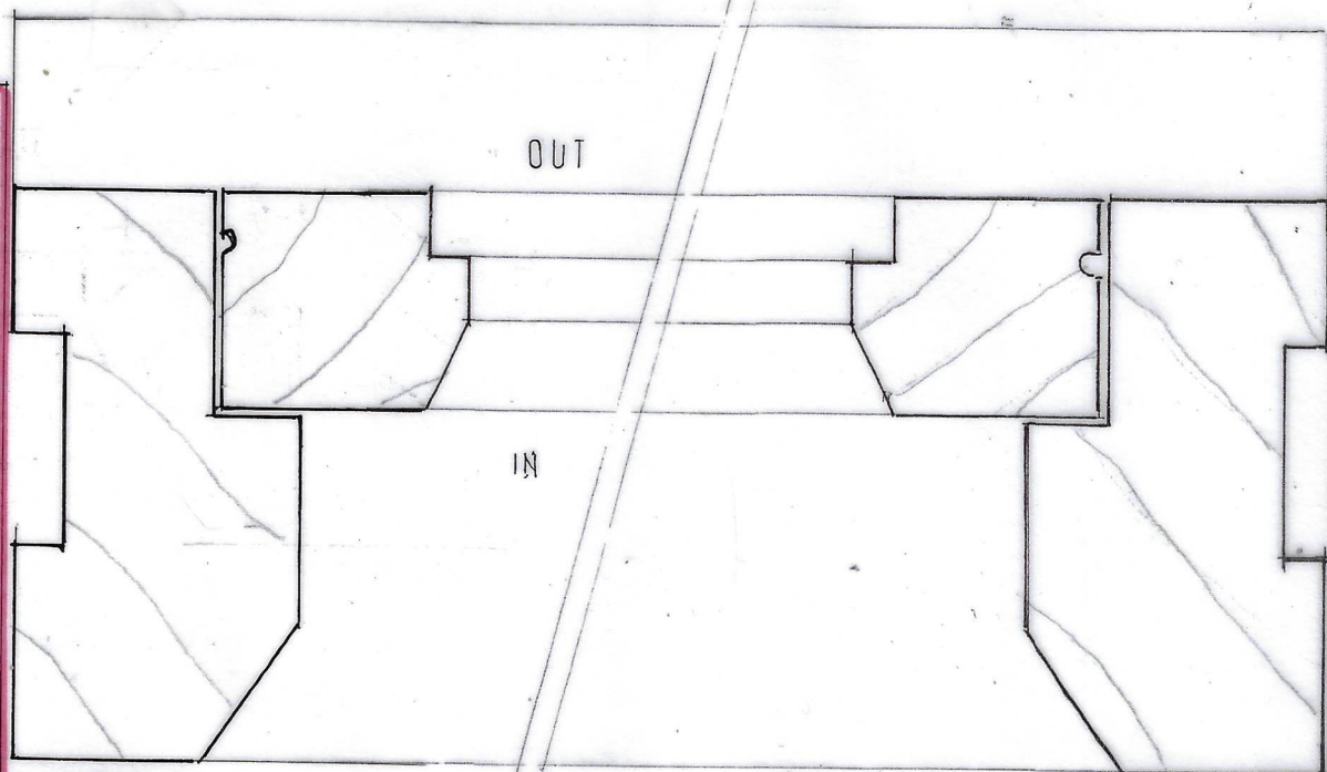
Half Full Size Plan - single casement
