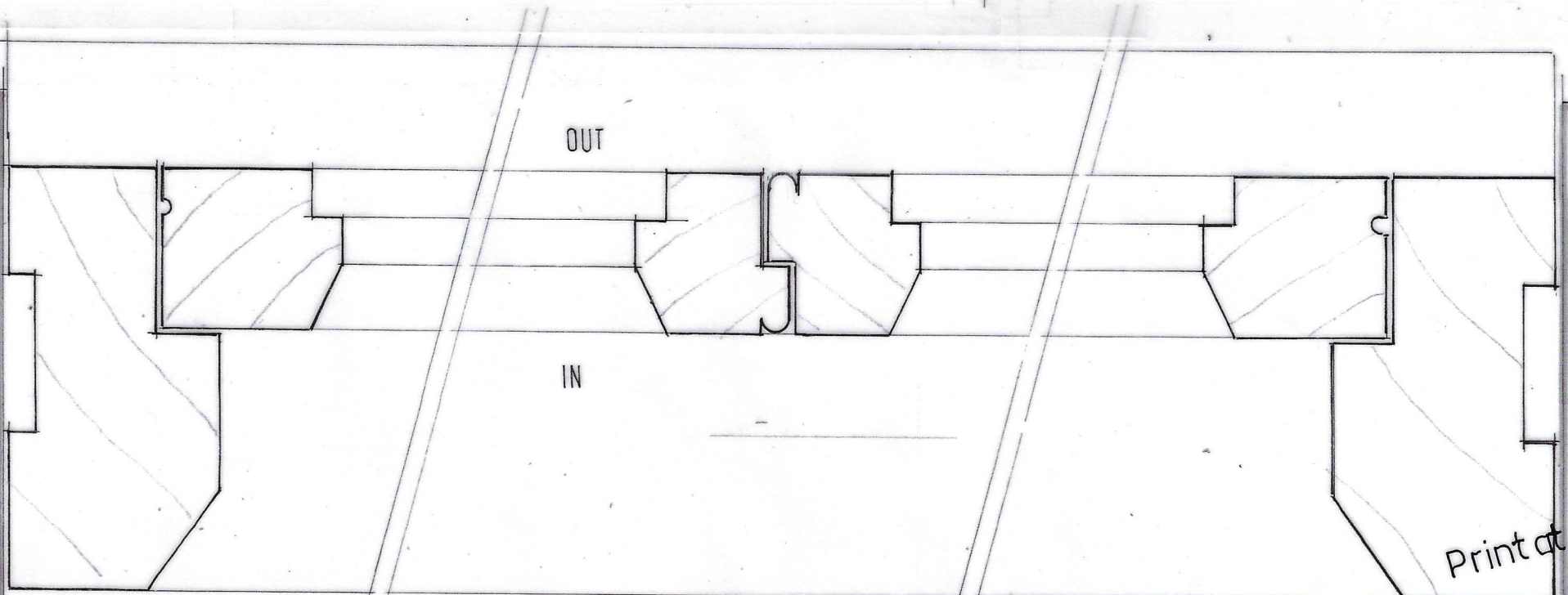
Half Full Size Plan DRAFT SEALS NOT SHOWN
