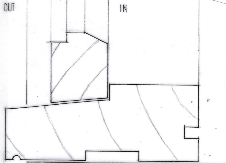
Half Full Size Section DRAFT SEALS NOT SHOWN
