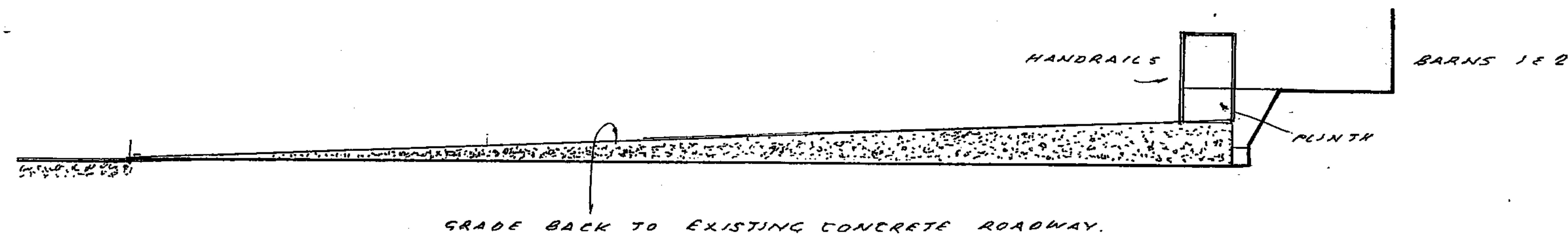
SECTION THROUGH CARPORT AND PLINTH. SCALE 1:100.
