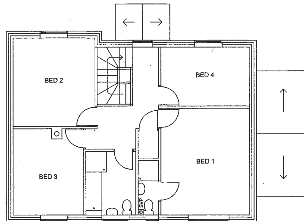
PROPOSED FIRST FLOOR PLAN - PLOTS 2&3
