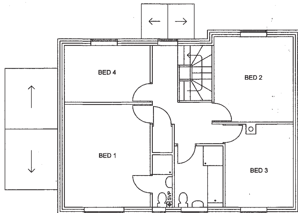
PROPOSED FIRST FLOOR PLAN - PLOT 1
