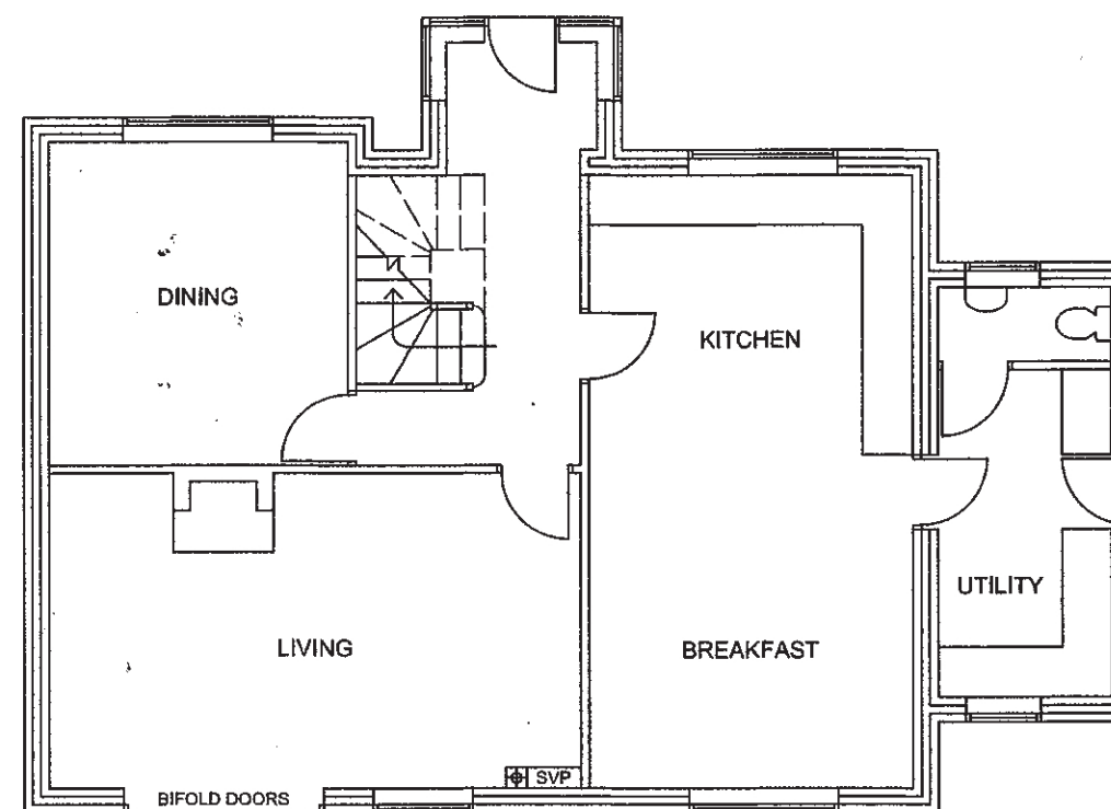
PROPOSED GROUND FLOOR PLAN - PLOTS 2&3
