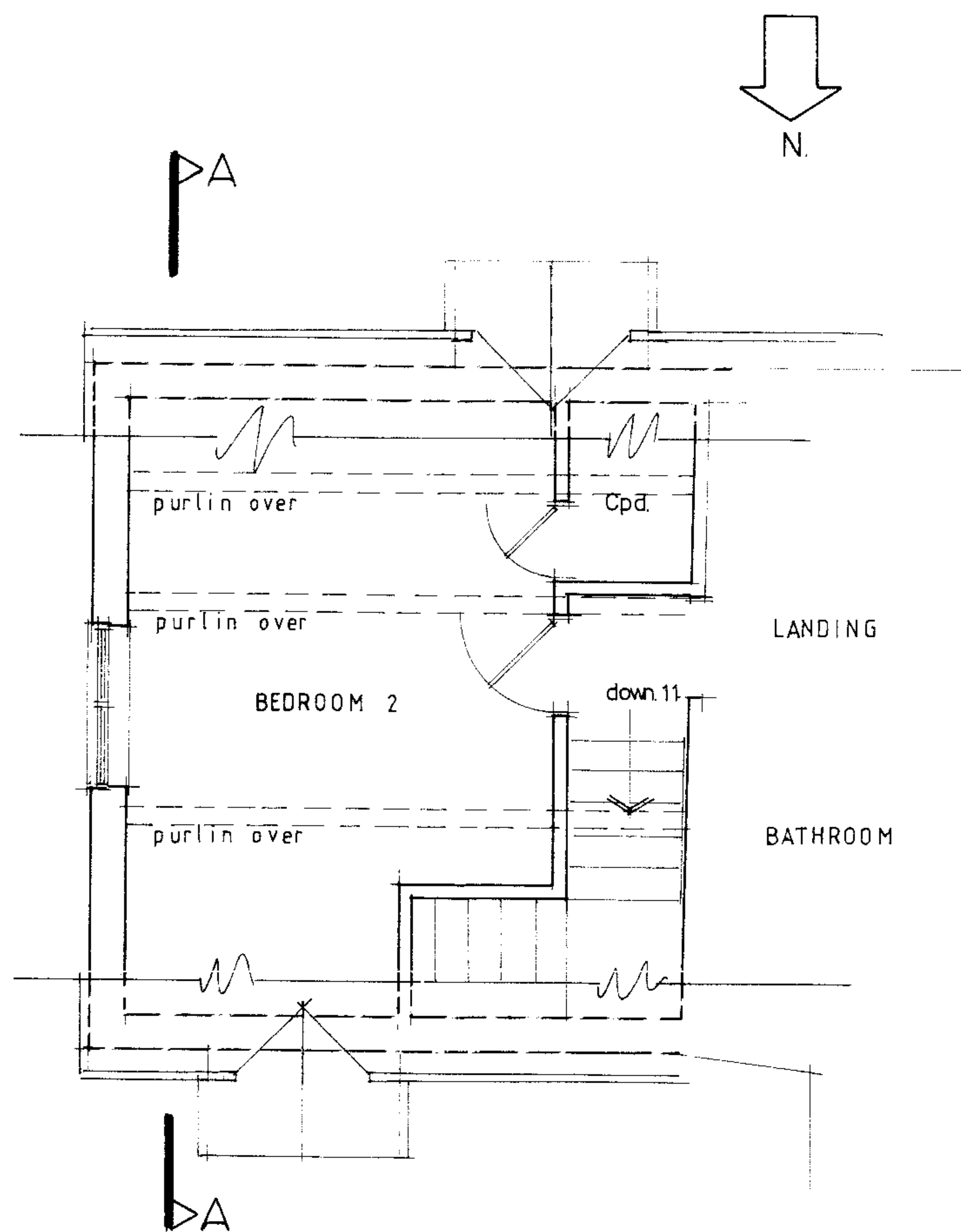
PART FIRST FLOOR PLAN. 1:50.
