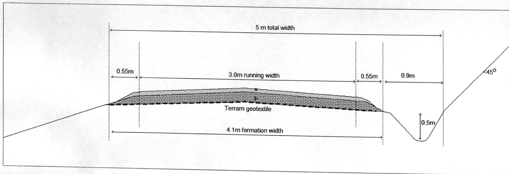
Drawing 1: Standard Haul Road
