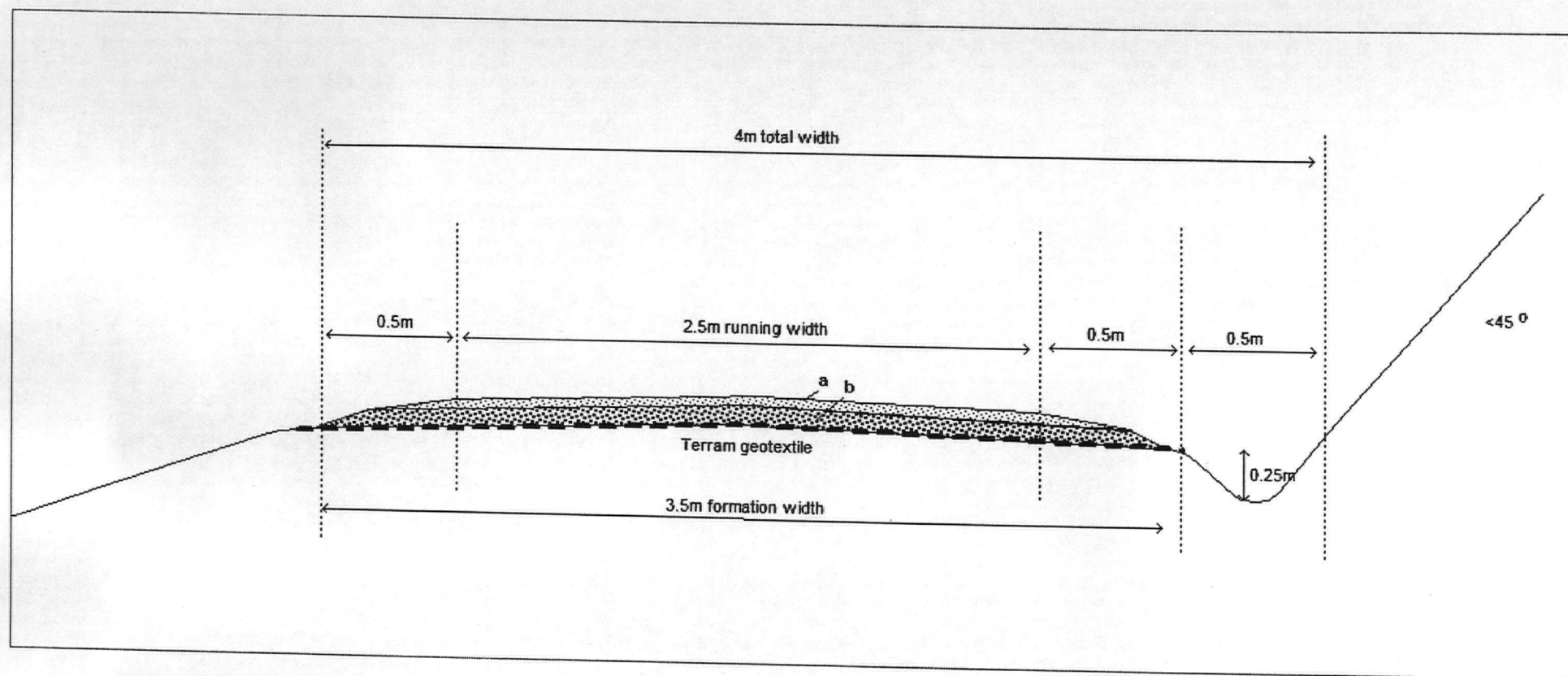
Drawing 2: Narrow Haul Road
