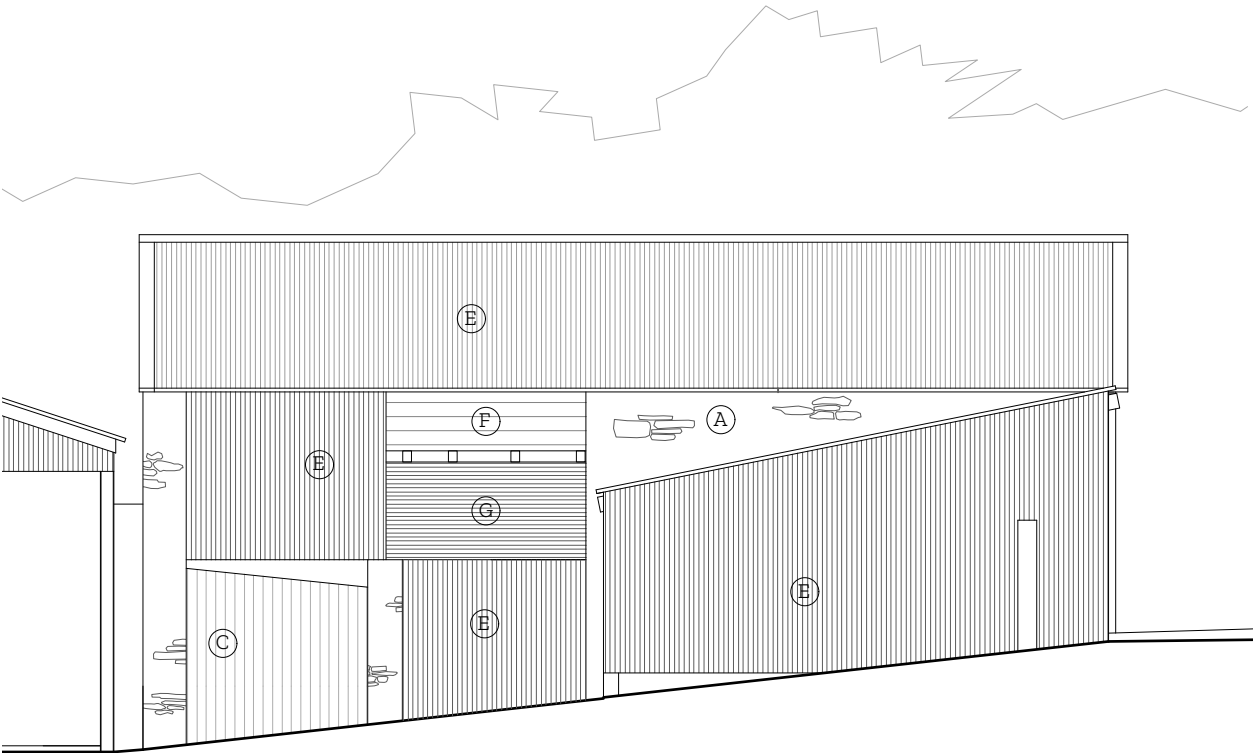
1:100 East Elevation
