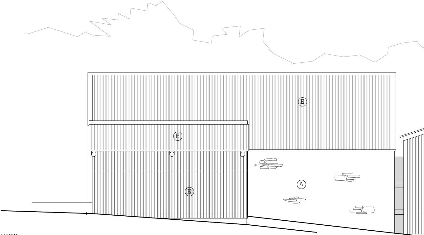
1:100 West Elevation
