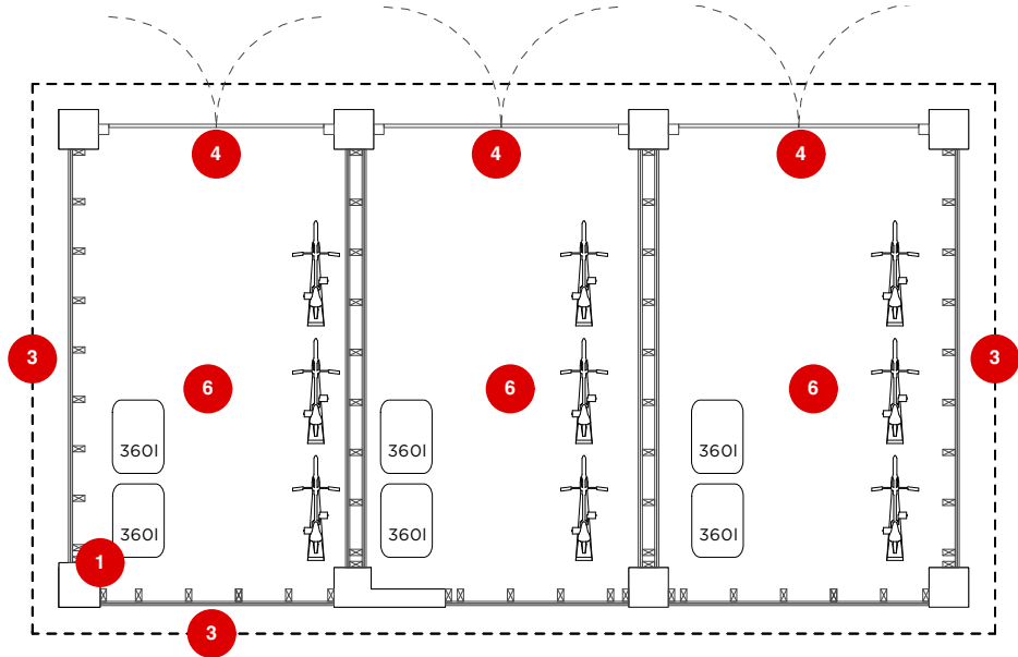
5 GROUND FLOOR PLAN - PROPOSED SCALE - 1:100
