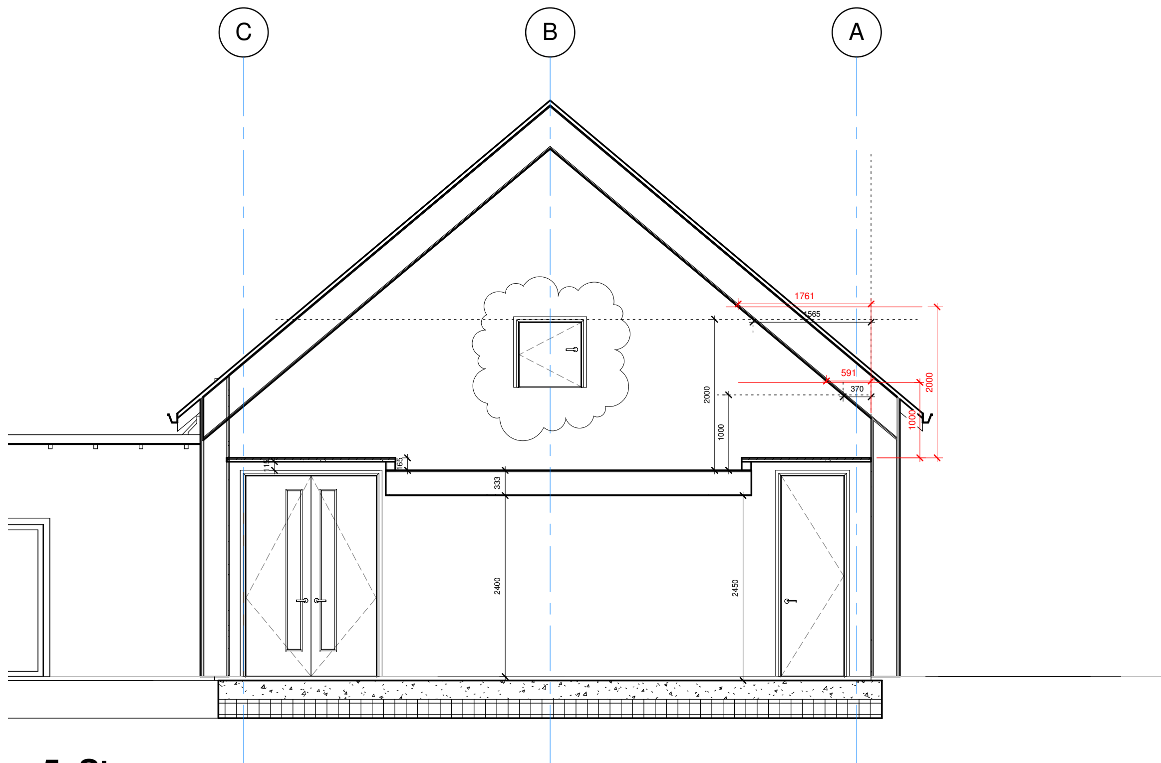
Section 5: Store 1 : 50
