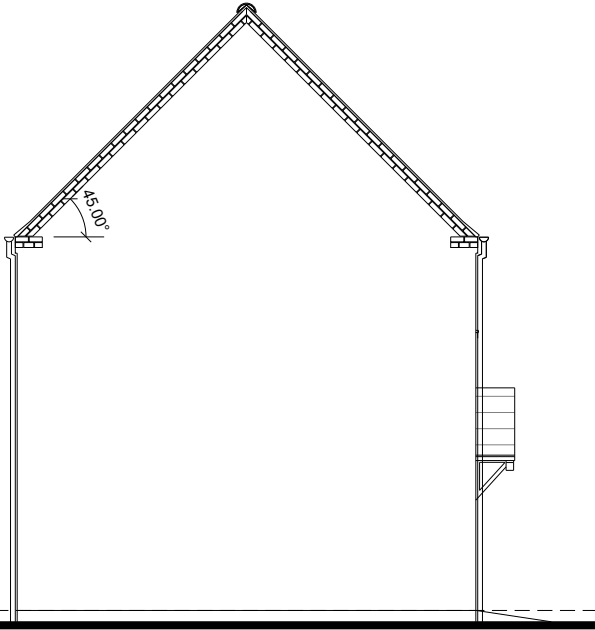
LEFT ELEVATION
