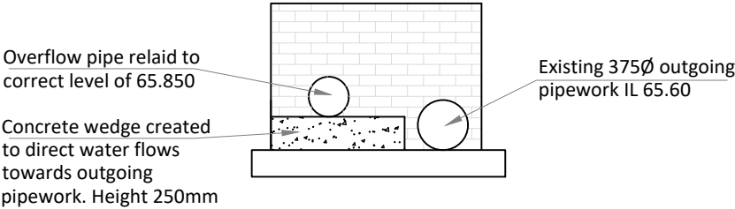
ELEVATIONAL VIEW 2-2 OF END WALLS
