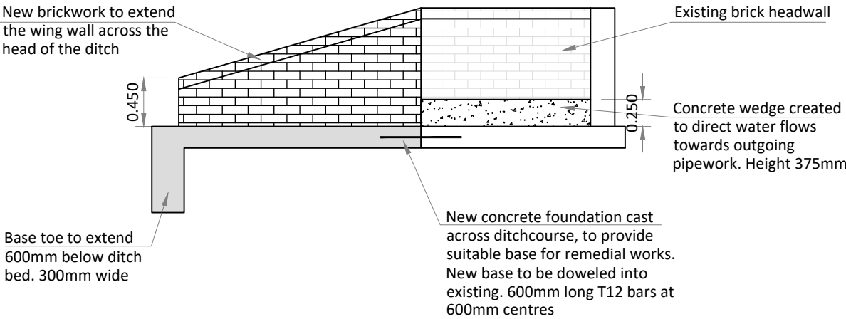
ELEVATIONAL VIEW 1-1 OF WING WALLS
