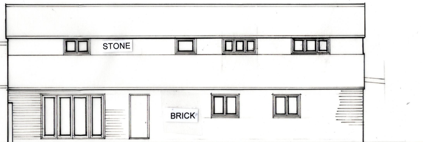
02 WEST ELEVATION
