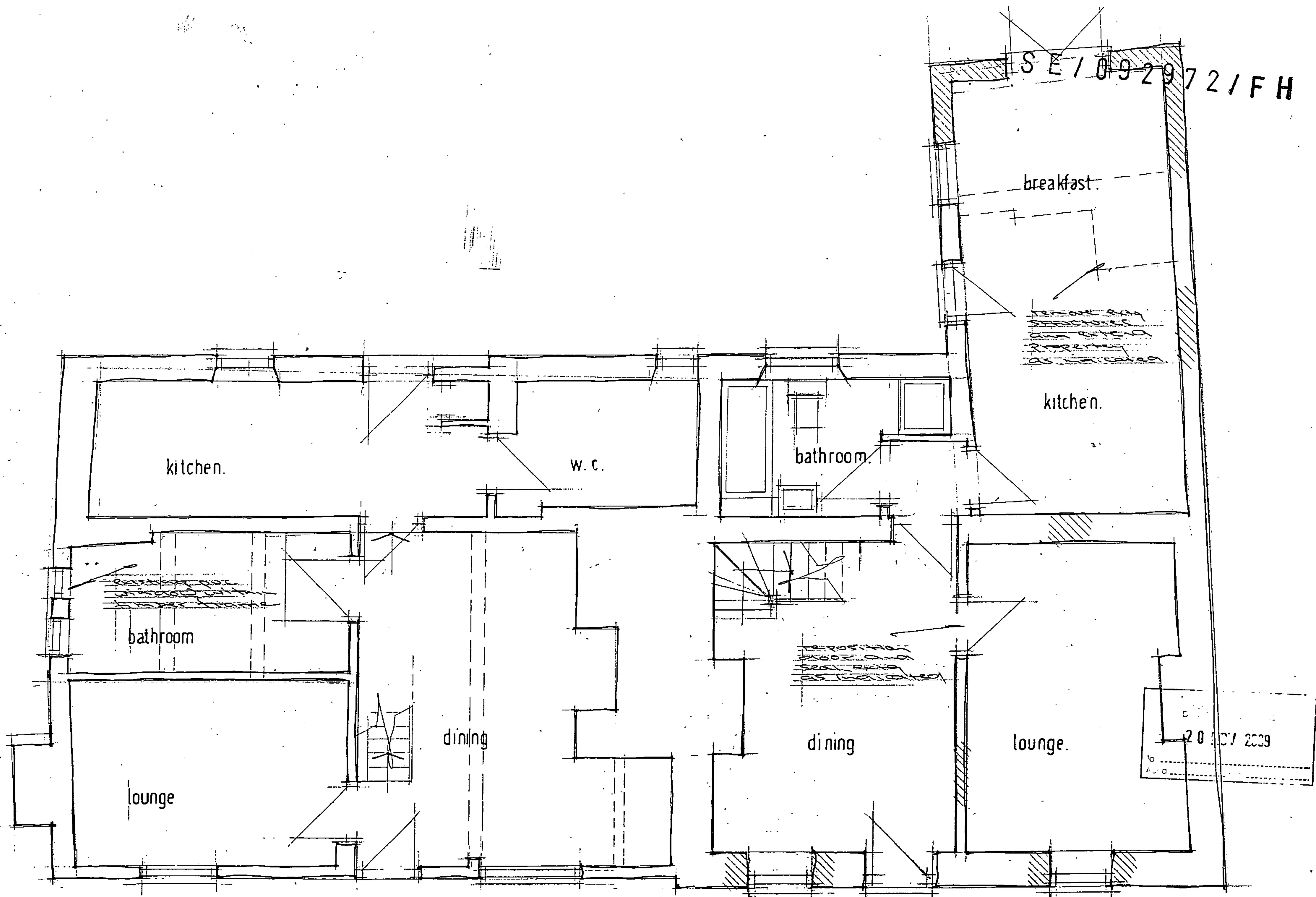
proposed ground floor plan.
