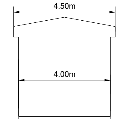
Left Elevation
