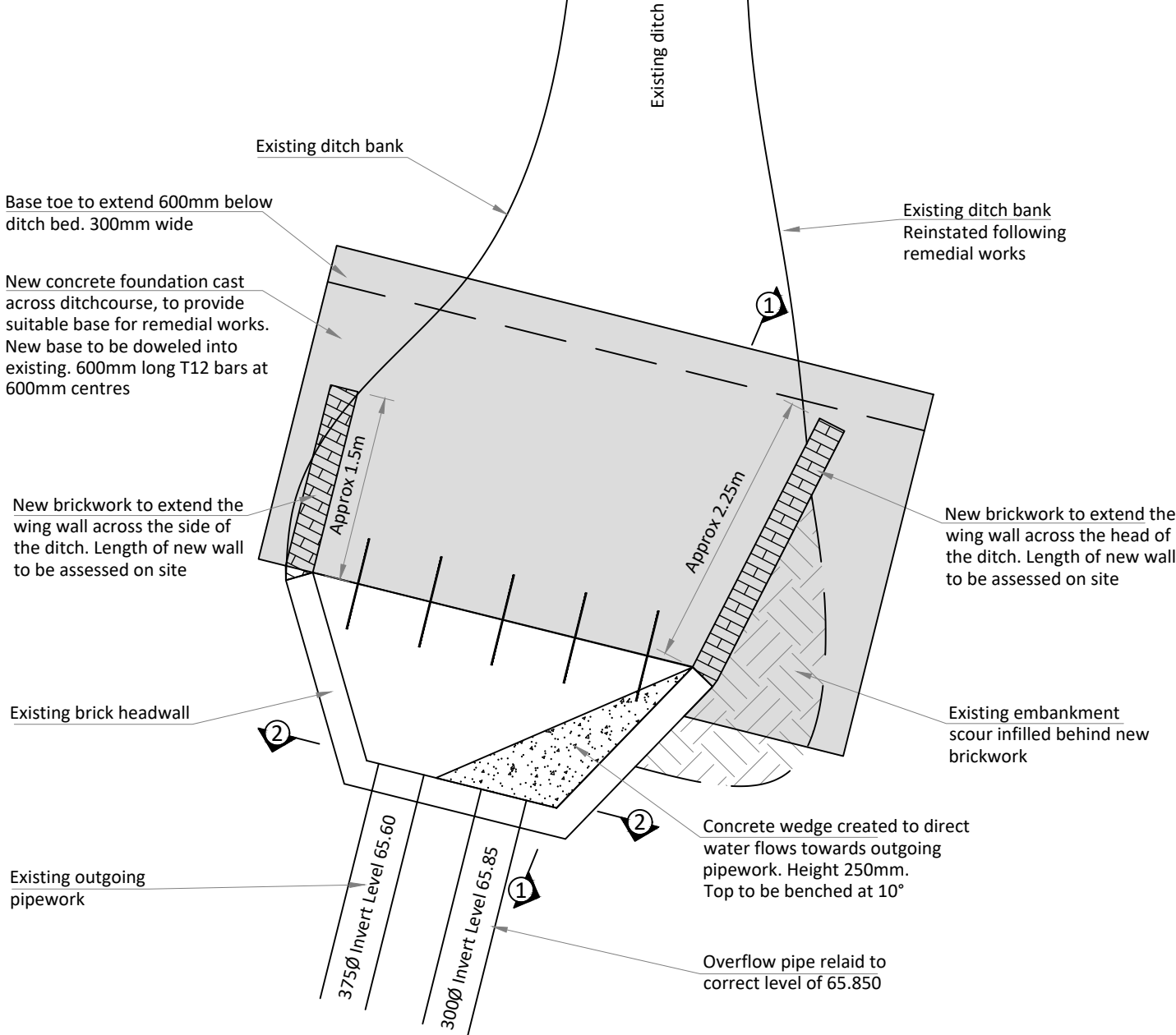
PLAN VIEW OF HEADWALL
