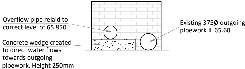
ELEVATIONAL VIEW 2-2 OF END WALLS
