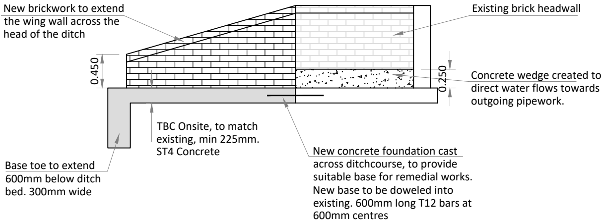
ELEVATIONAL VIEW 1-1 OF WING WALLS
