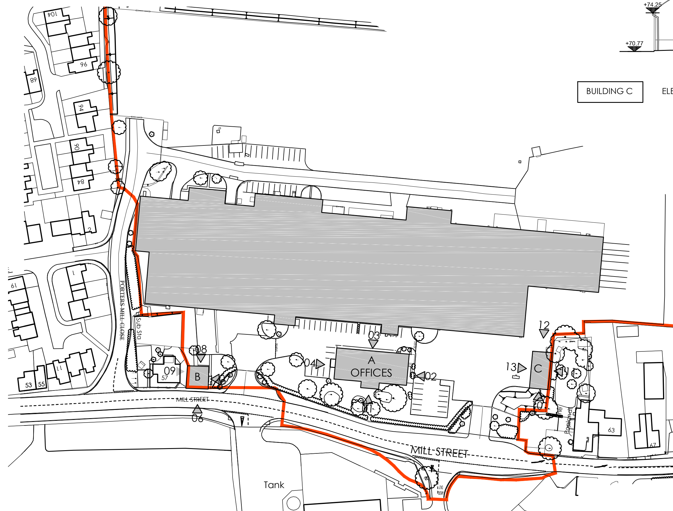
LOCATION PLAN @ 1:1000
