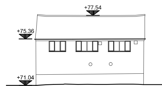
BUILDING B
