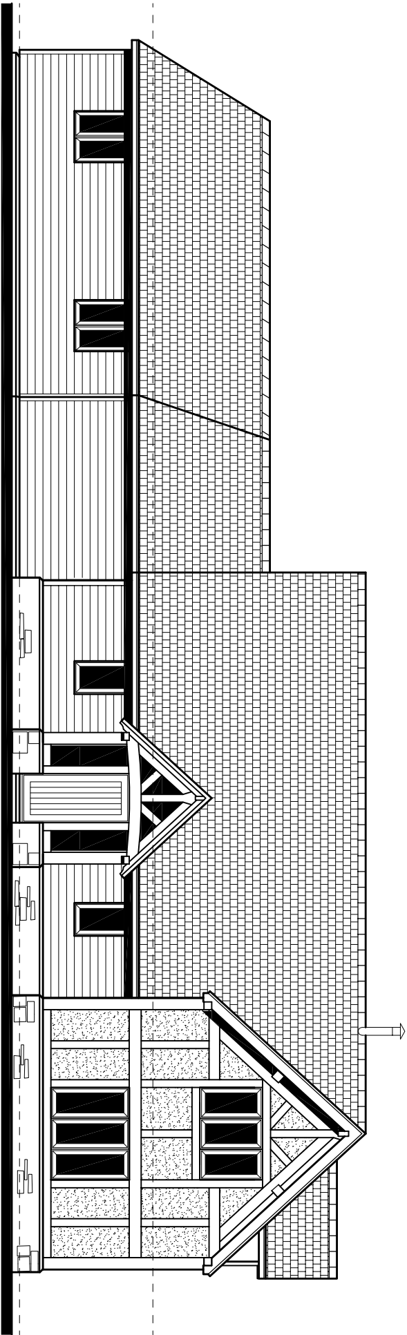
FRONT ELEVATION
