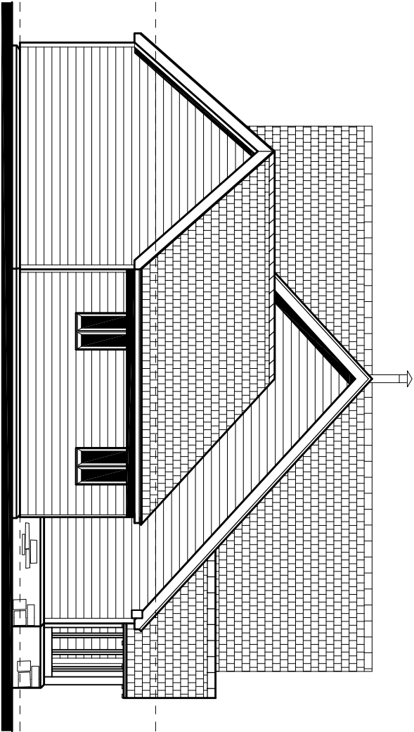
SIDE ELEVATION
