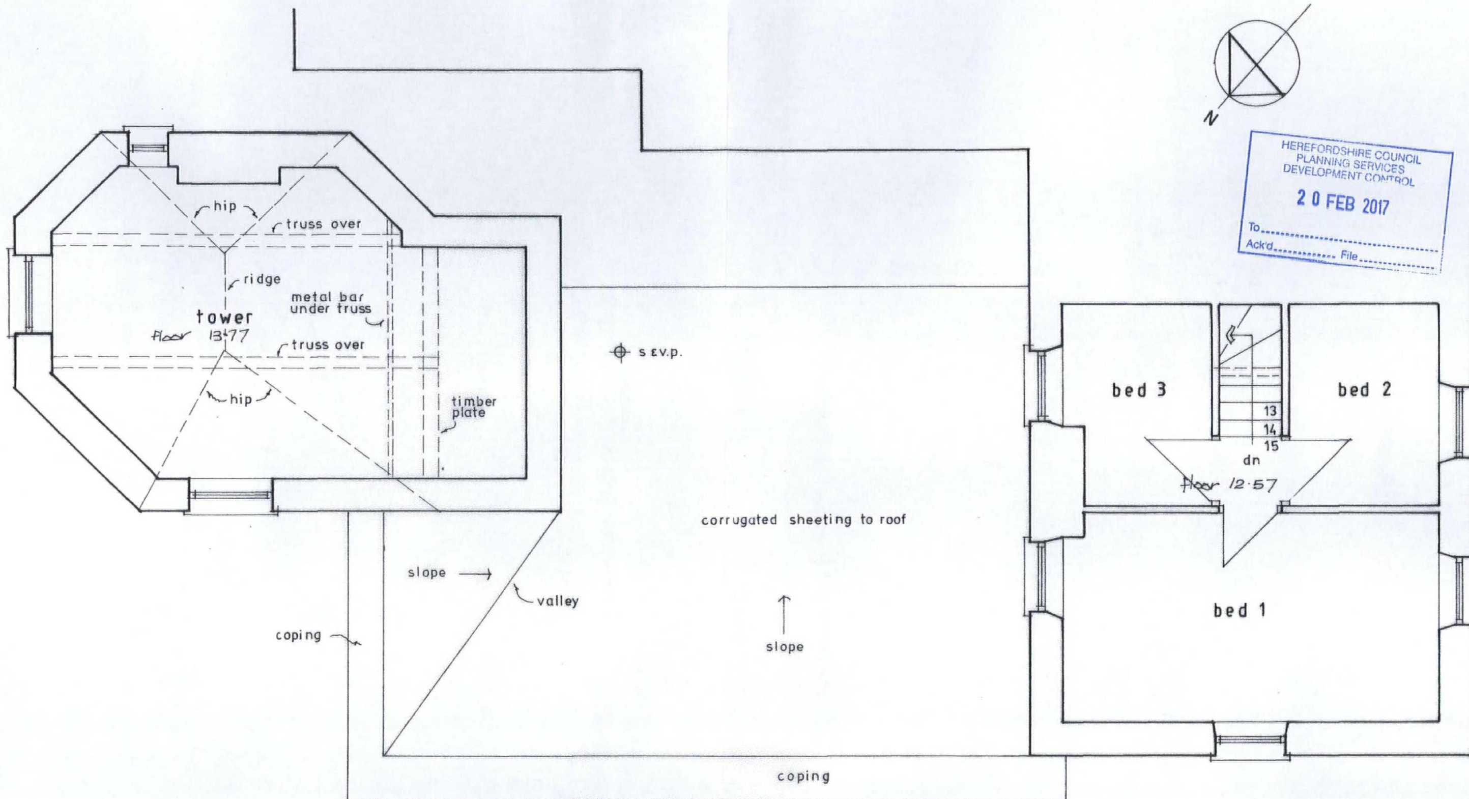
First Floor Plan scale 1:50
