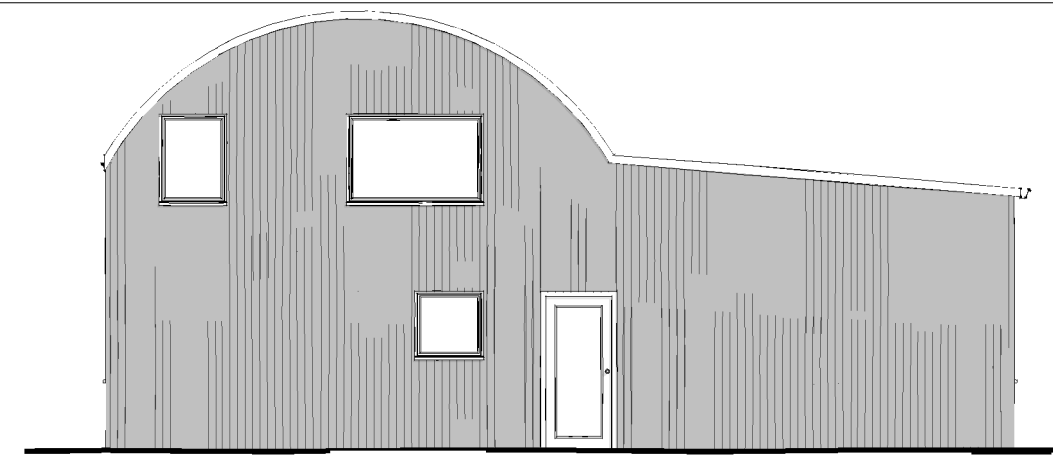
4 Barn C north proposed 1 : 100
