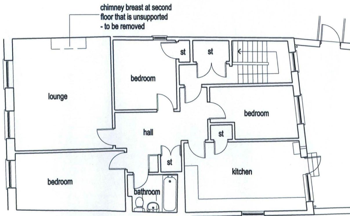
Part Second Floor Layout
