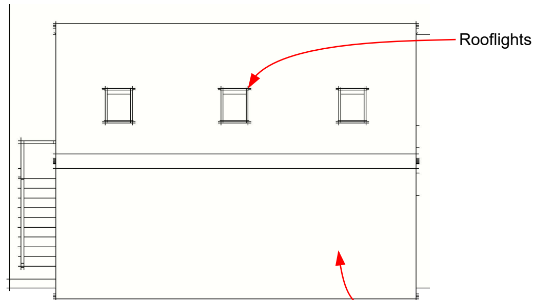
ROOF PLAN 1:100
