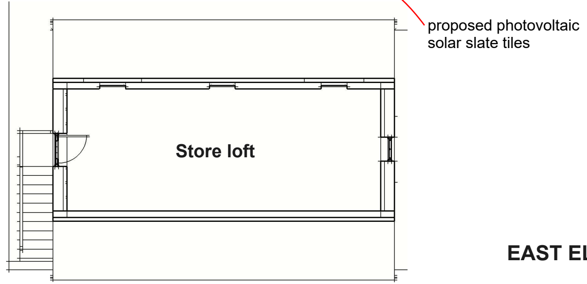
FIRST FLOOR 1:100
