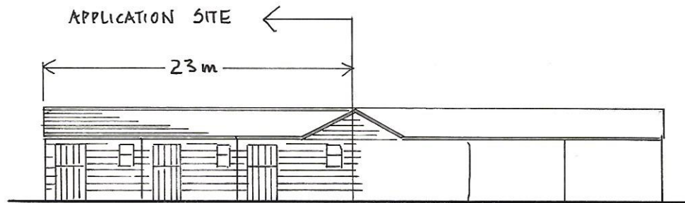
FRONT (NORTH) ELEVATION (1:200)
