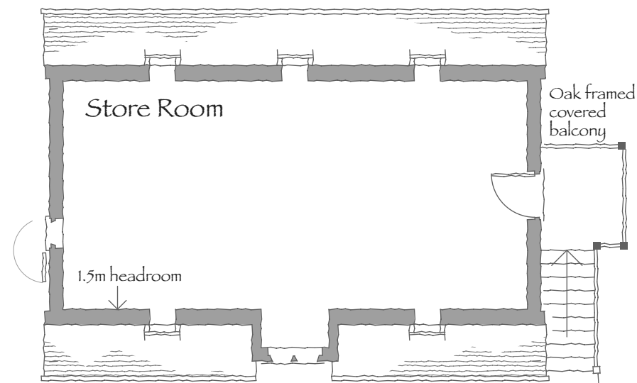
ATTIC PLAN
