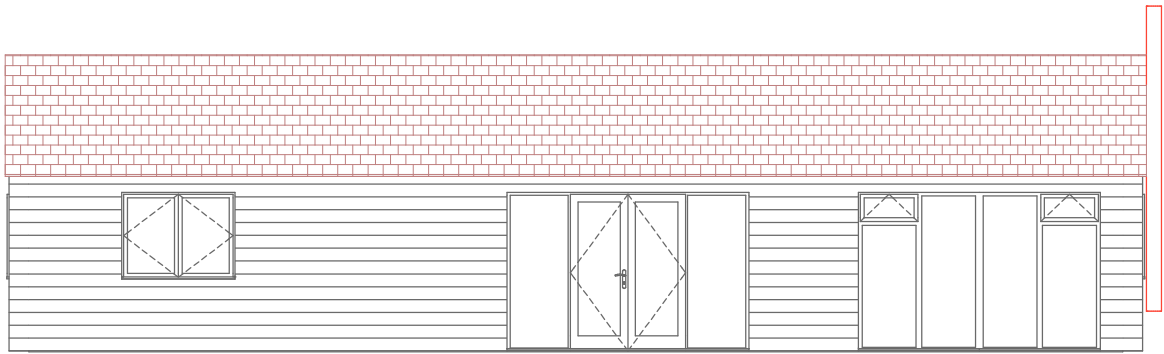
North Elevation 1:100
