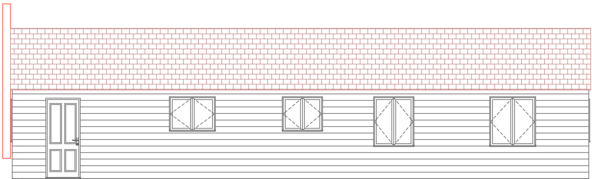
South Elevation 1:100
