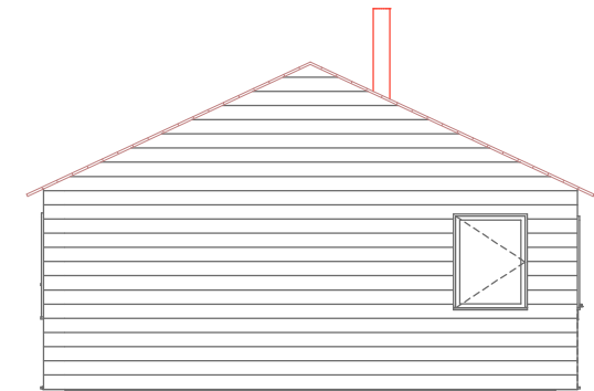
East Elevation 1:100
