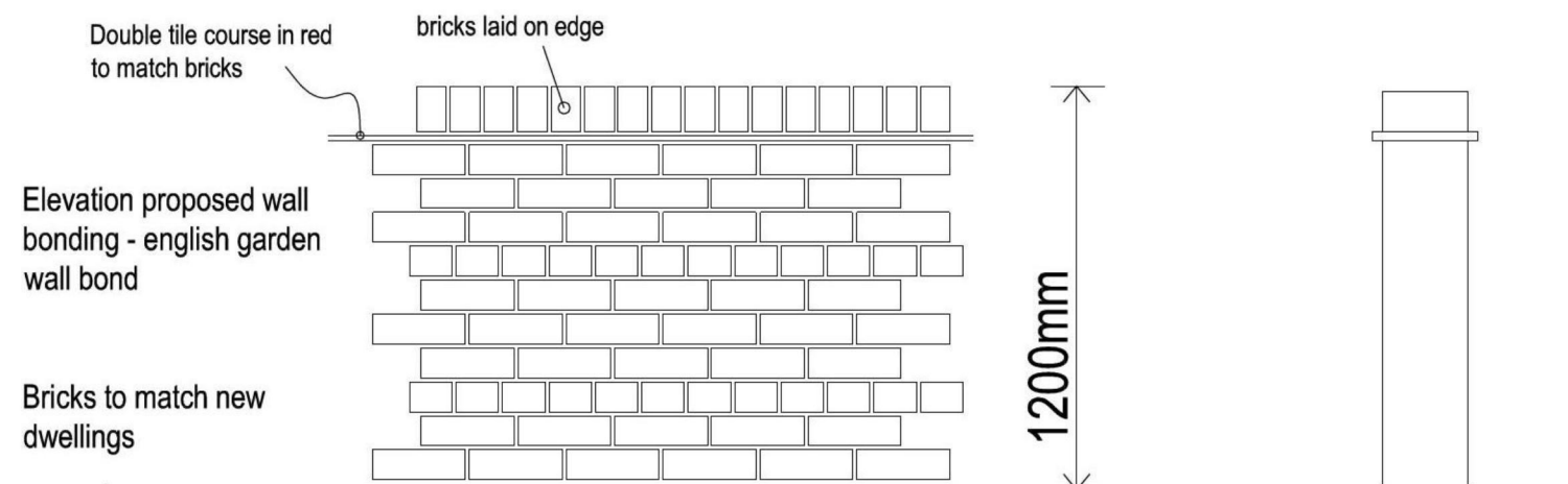
WALL DETAILS - SAME FOR BOTH 1.2m & 2m HIGH WALLS. 1/20
