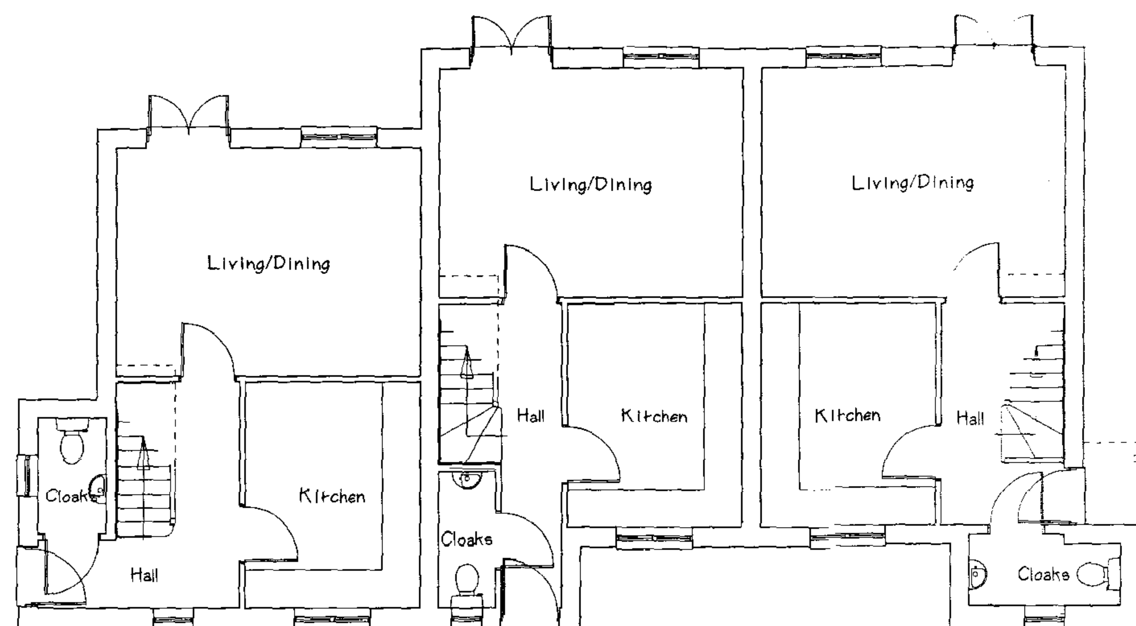
ground floor layout - units 1, 2 and 3.
