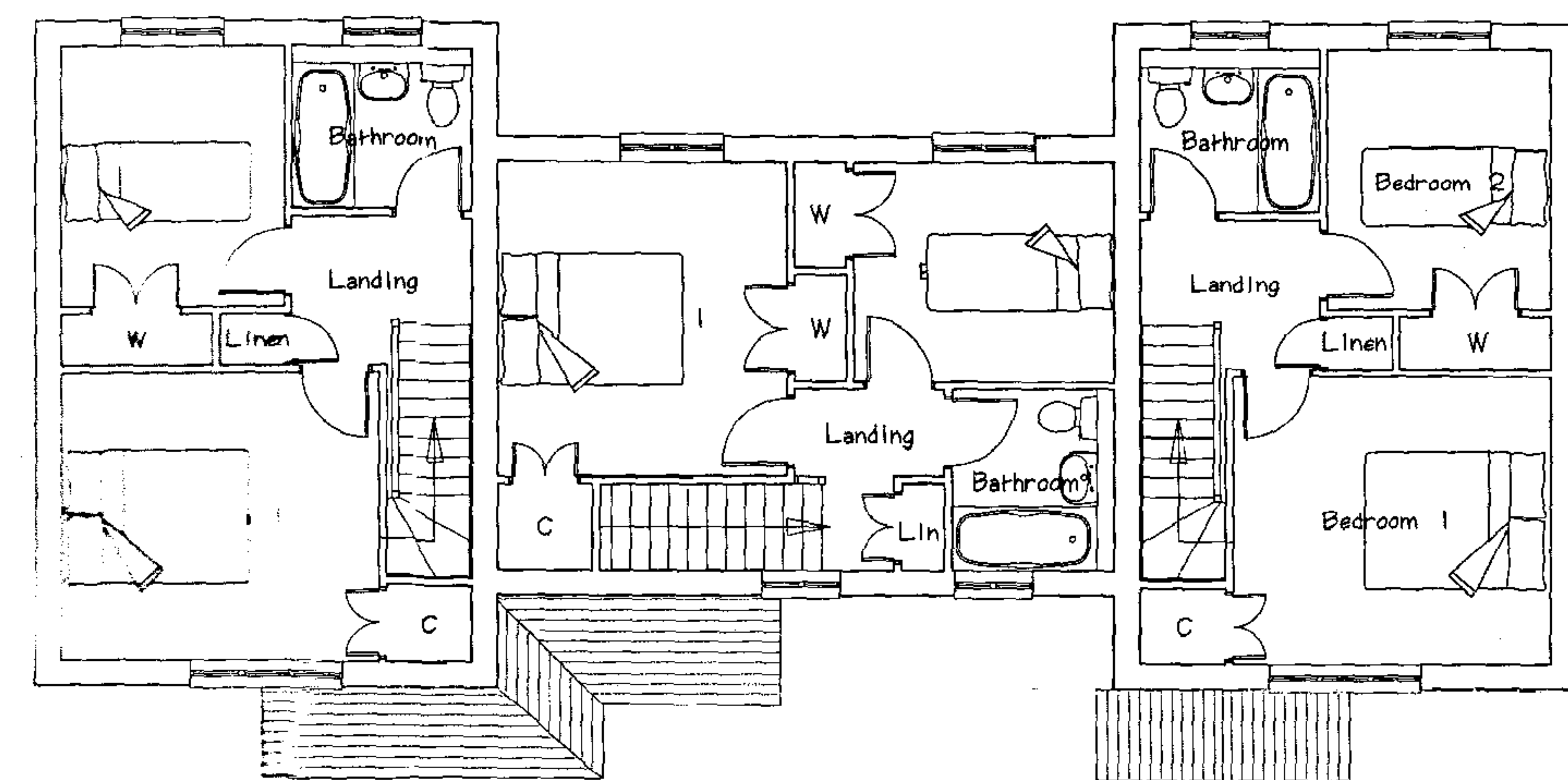
first floor layout - units 4, 5 and 6.
