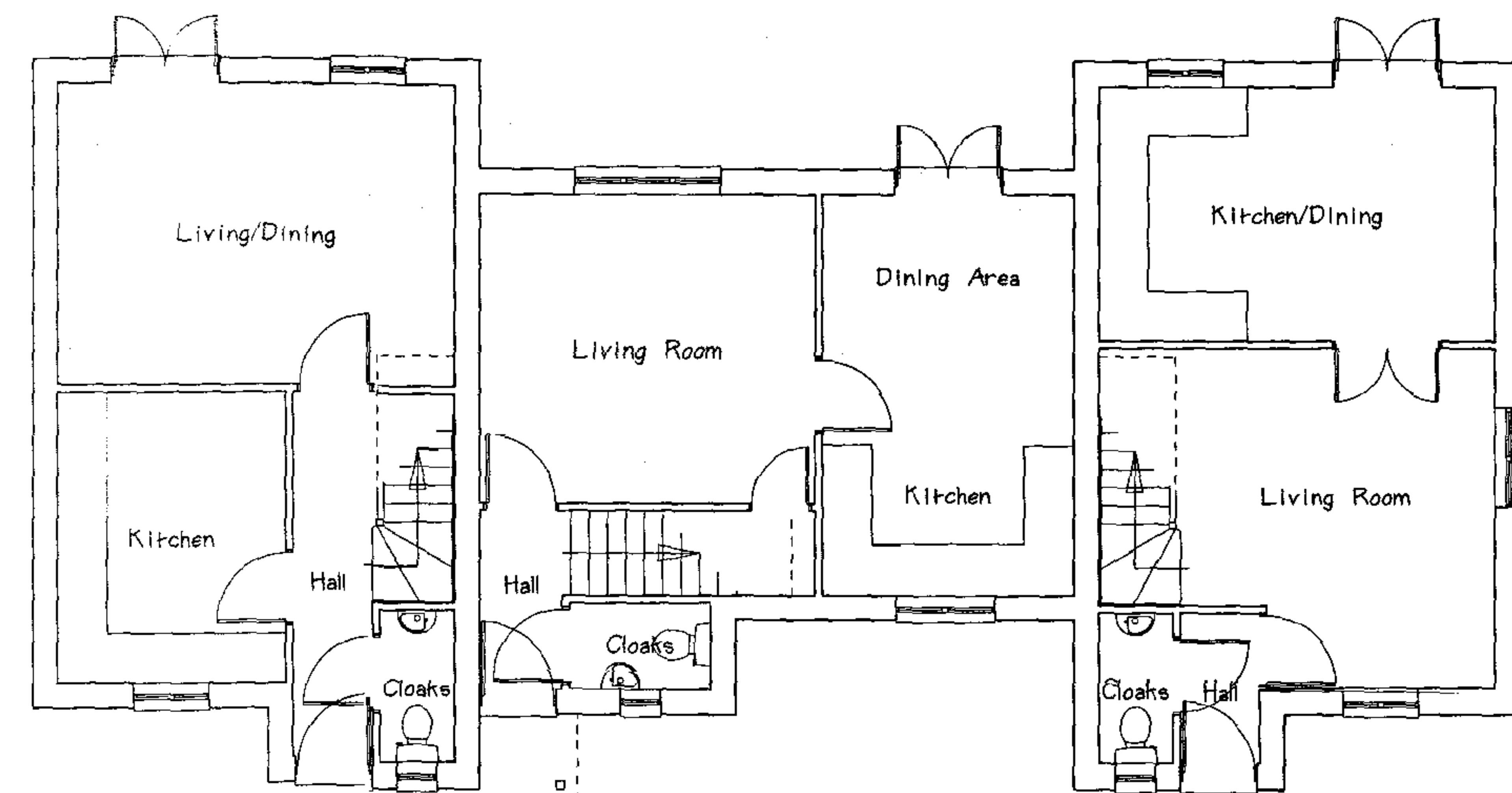
ground floor layout - units 4, 5 and 6.
