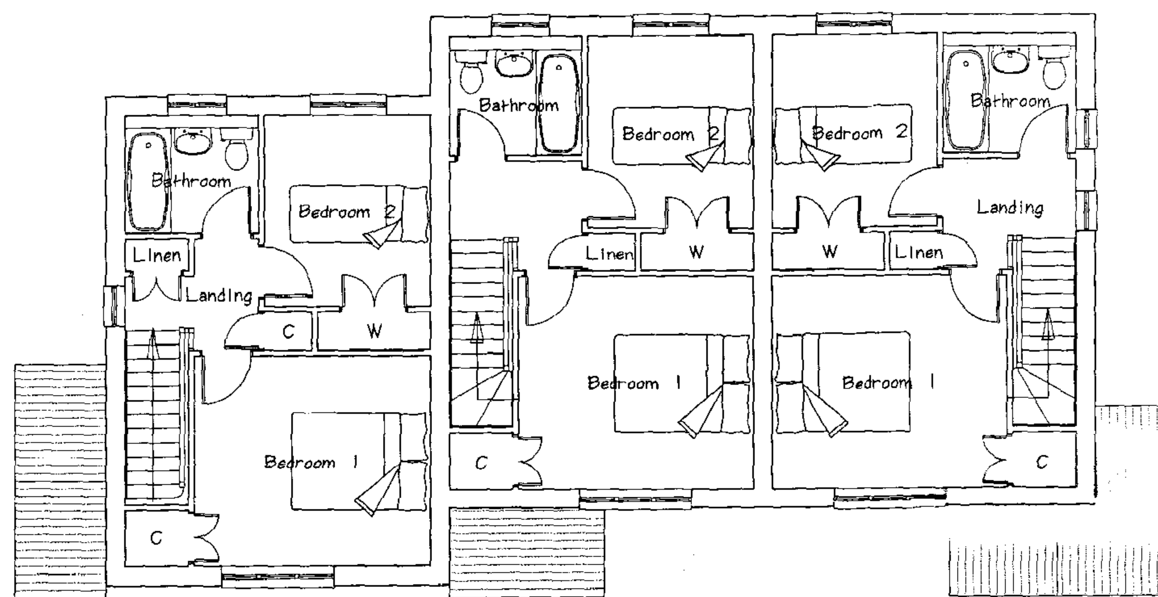
first floor layout - units 1, 2 and 3.
