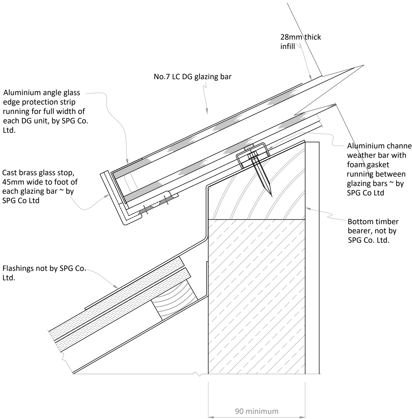
ROOFLIGHT BOTTOM DETAIL
