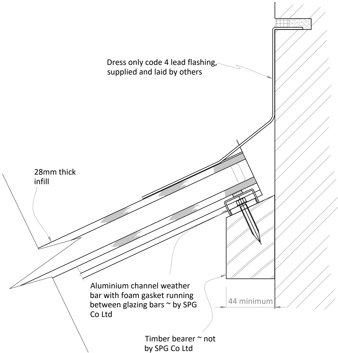
ROOFLIGHT ABUTMENT DETAIL
