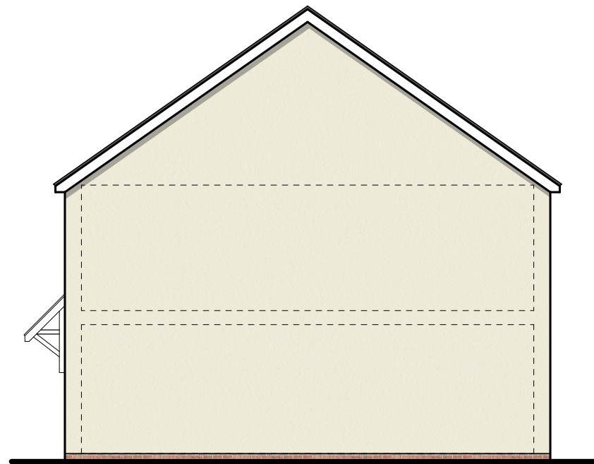
Plot 3 Side Elevation
