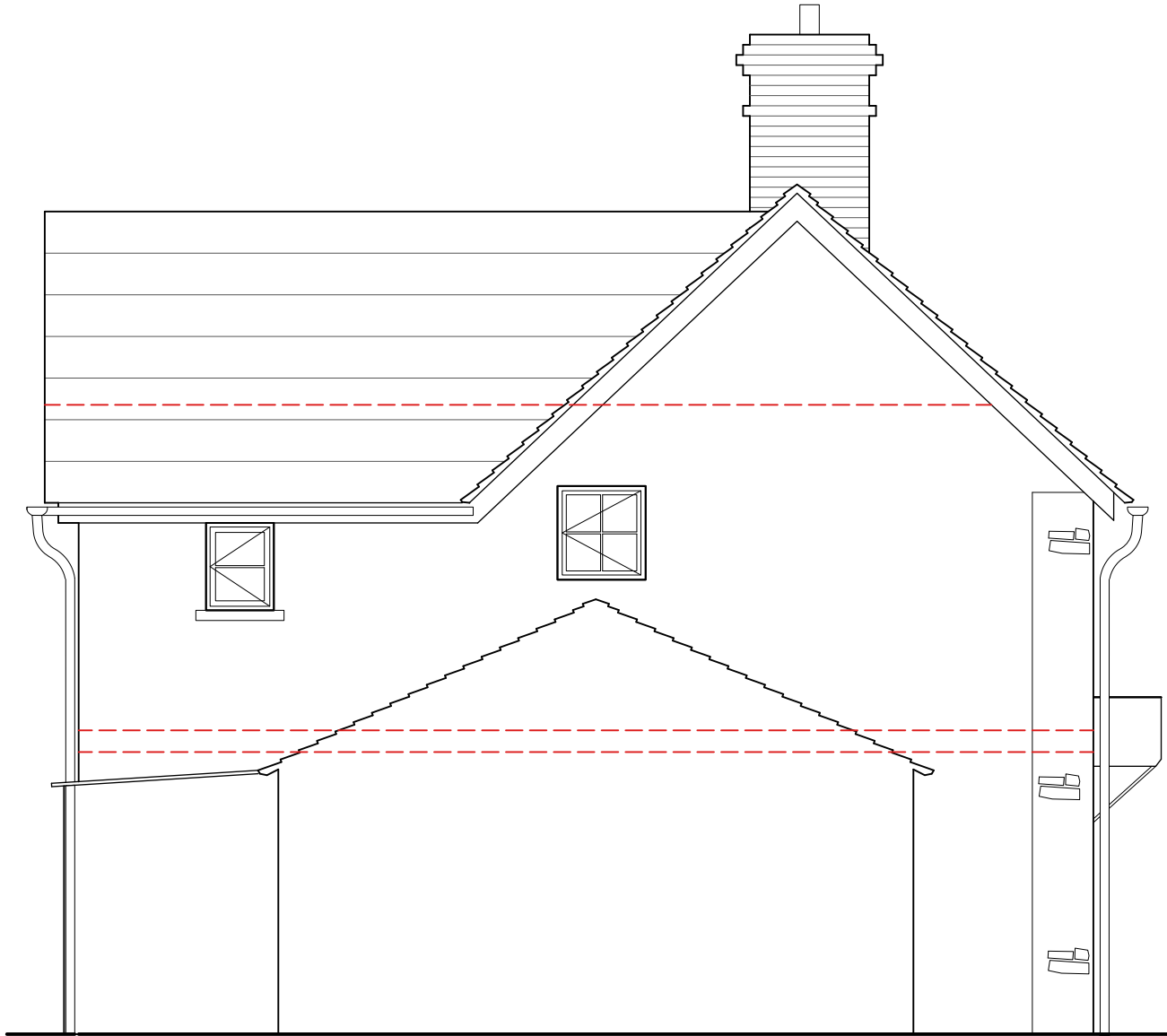
3 EXISTING SOUTH ELEVATION SCALE - 1:50
