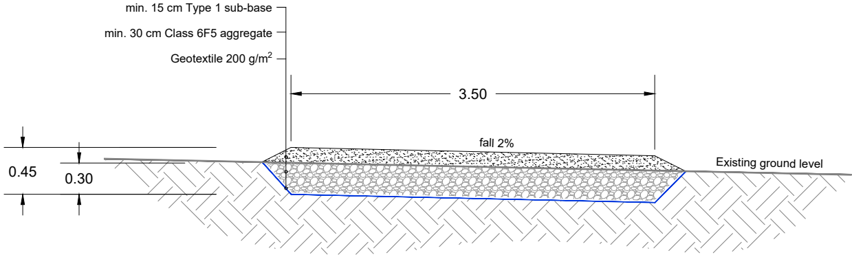
ACCESS TRACK - SLOPING GROUND
