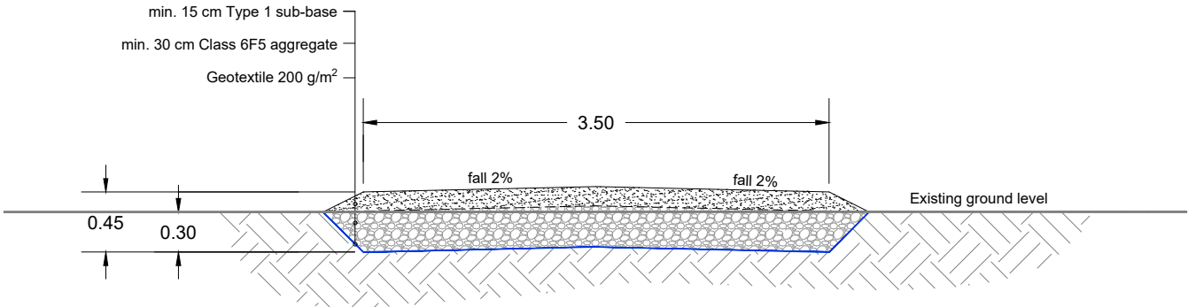
ACCESS TRACK - FLAT GROUND
