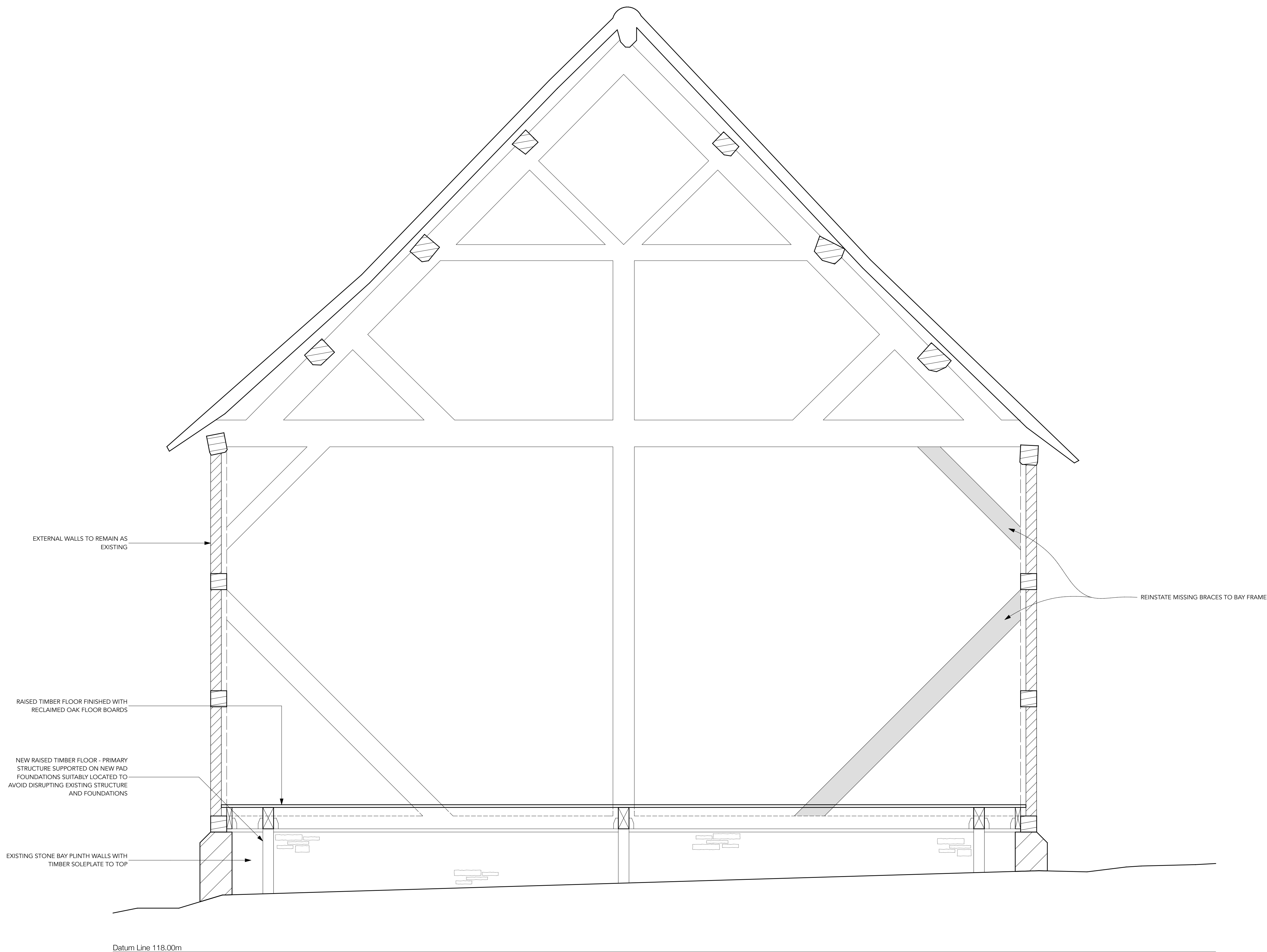
TYPICAL TRUSS AND BAY SECTION
