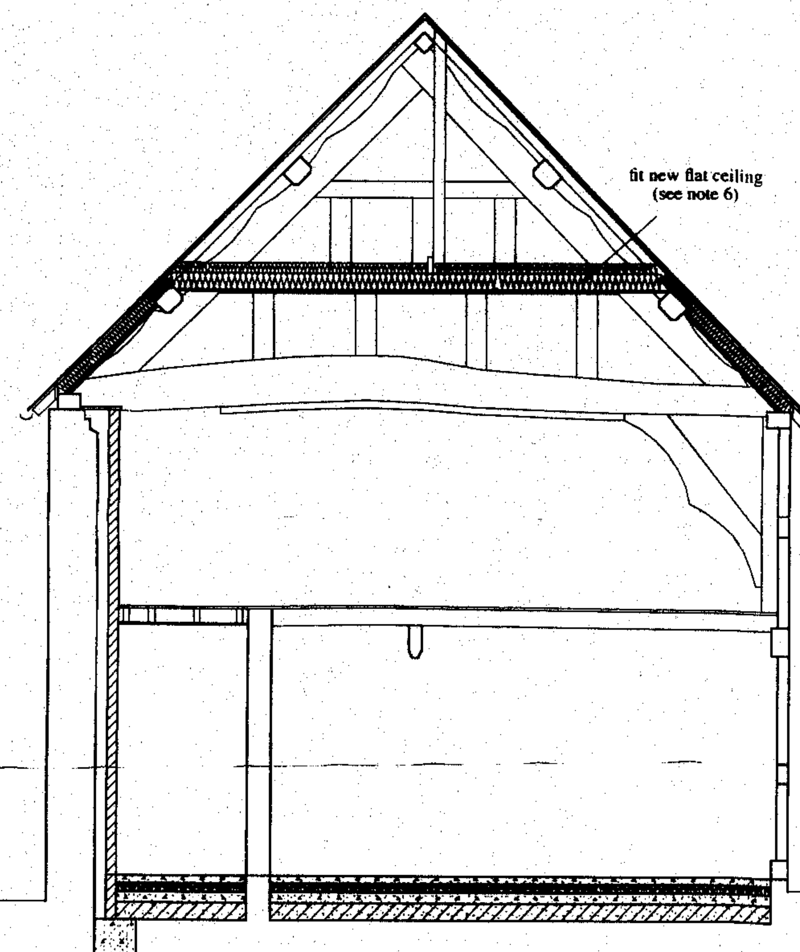
Section C-C
