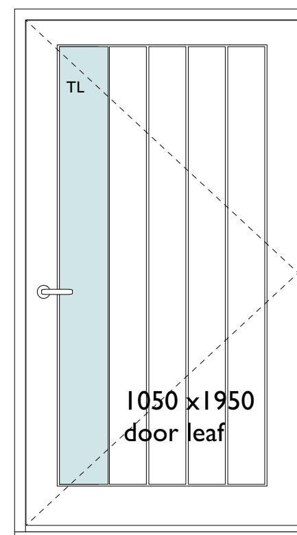
I No. D4.01 Solid oak frame and oak framed and boarded door with vision panel
