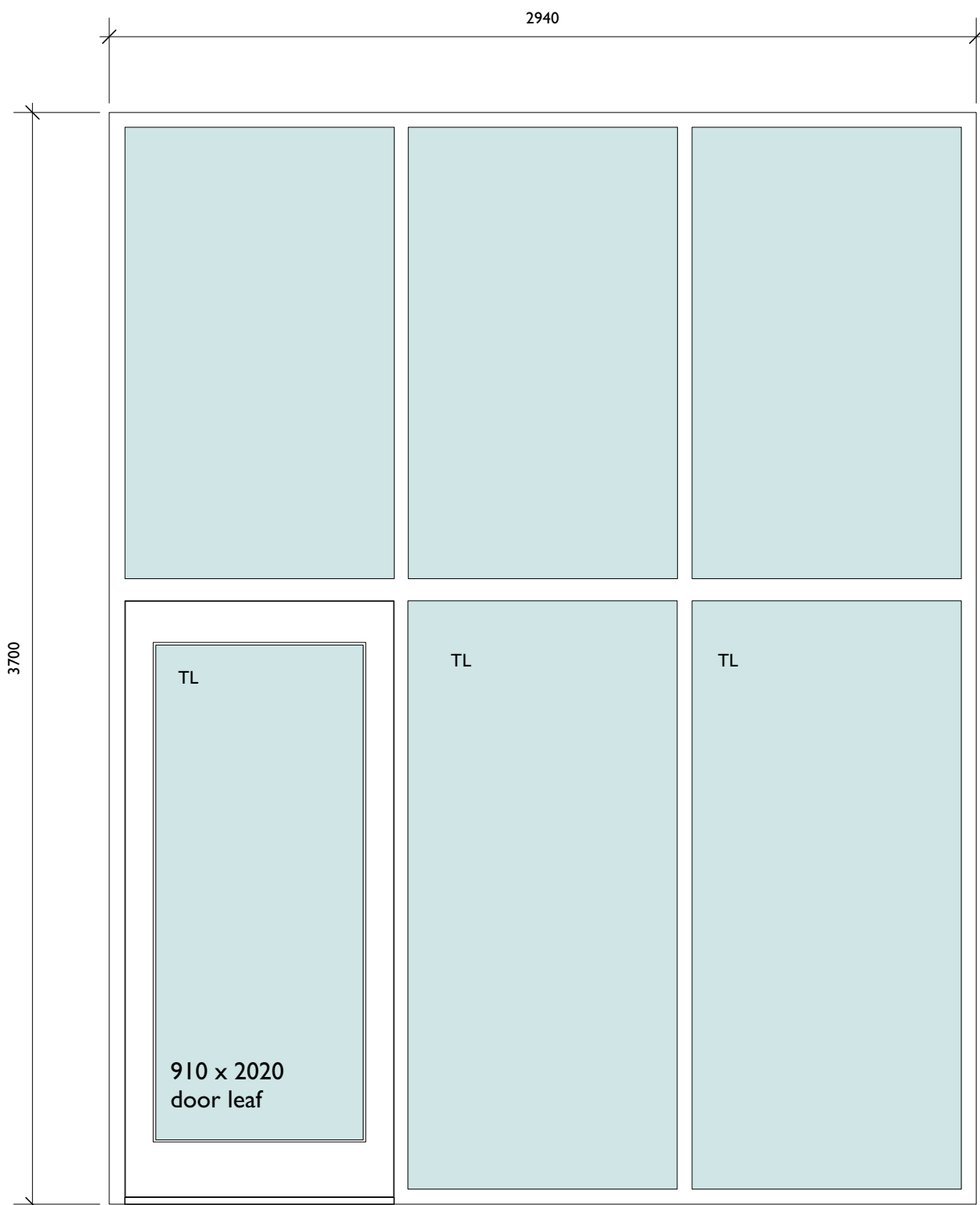
I No. W 2.01 with integral D 2.01 Engineered timber curtain wall and glazed door Units 2 & 4 External Doors
