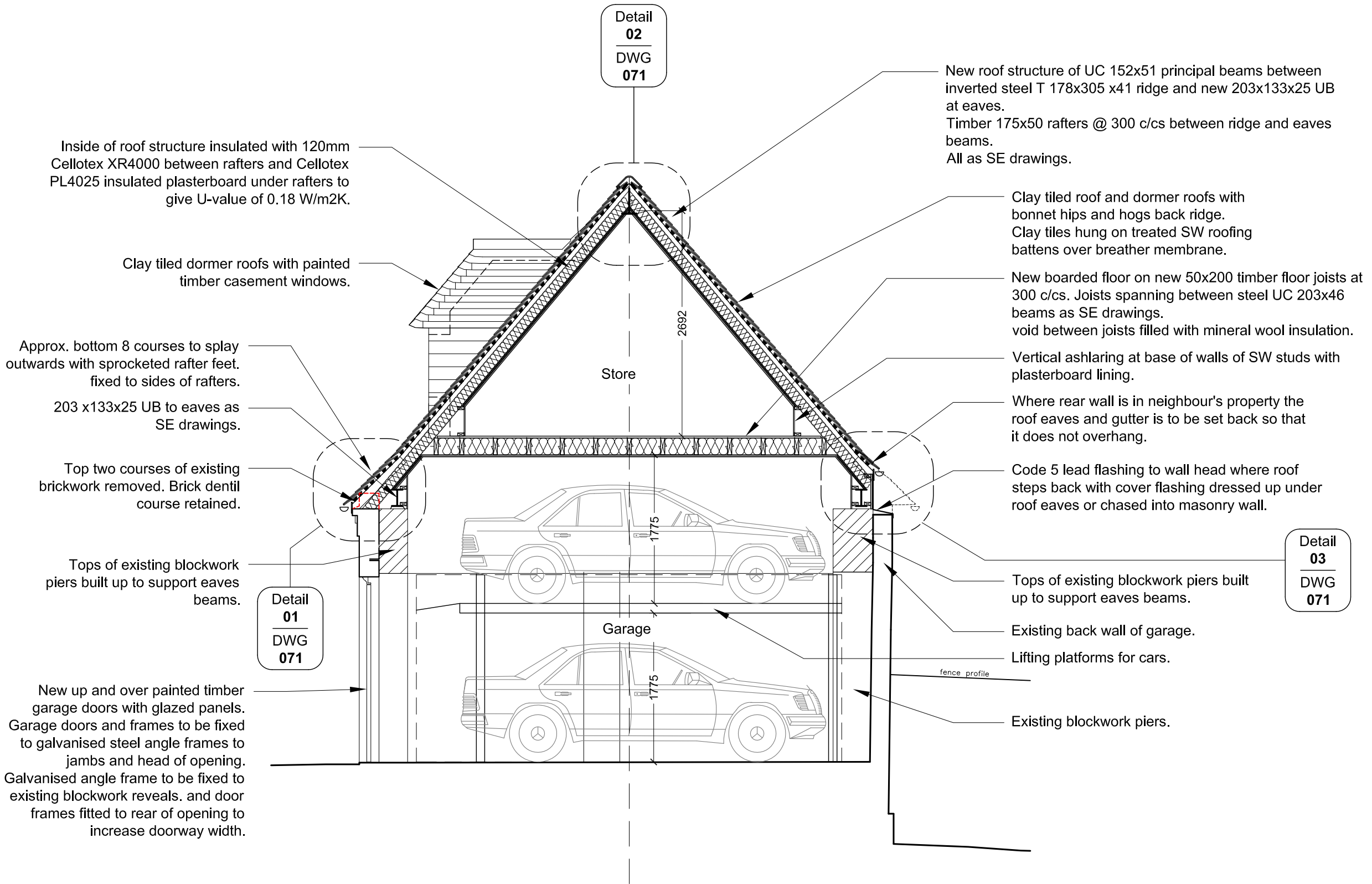
Section A - Scale 1:100
