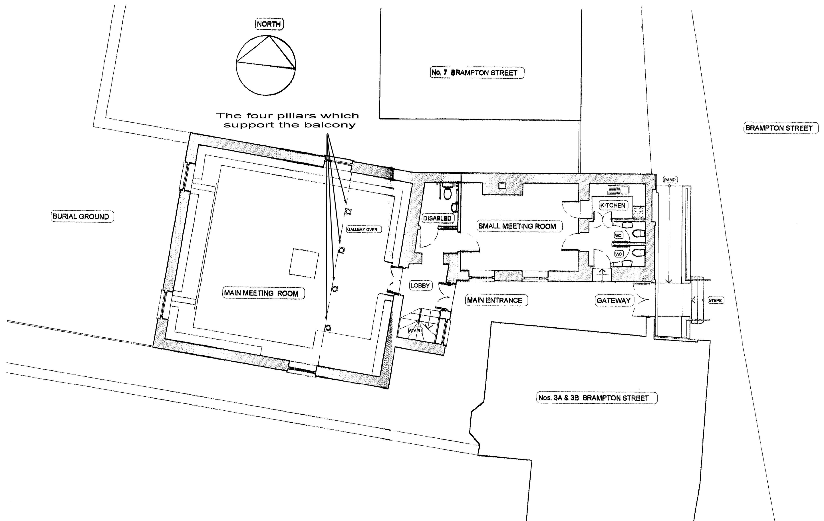
ROSS-ON-WYE QUAKER MEETING HOUSE : GROUND FLOOR PLAN
