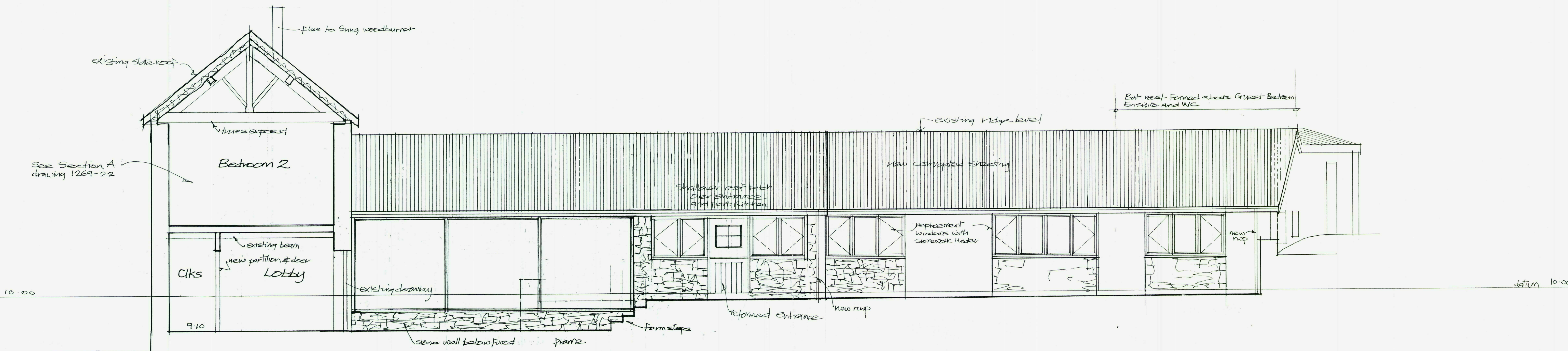
East Elevation - Barn Section
