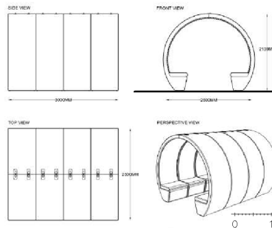
4, 8 PERSON POD 1:100
