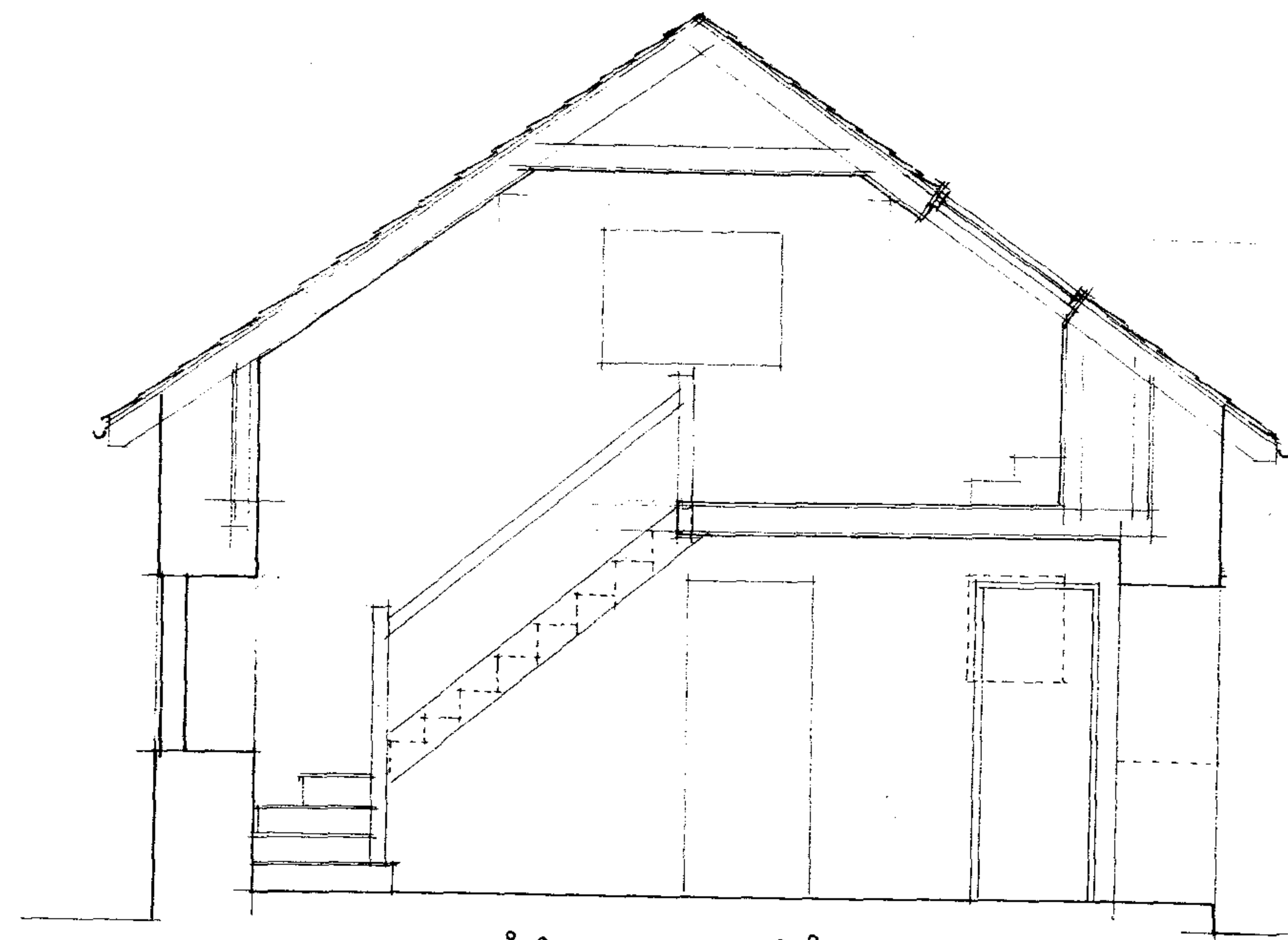
composite section 1:50
