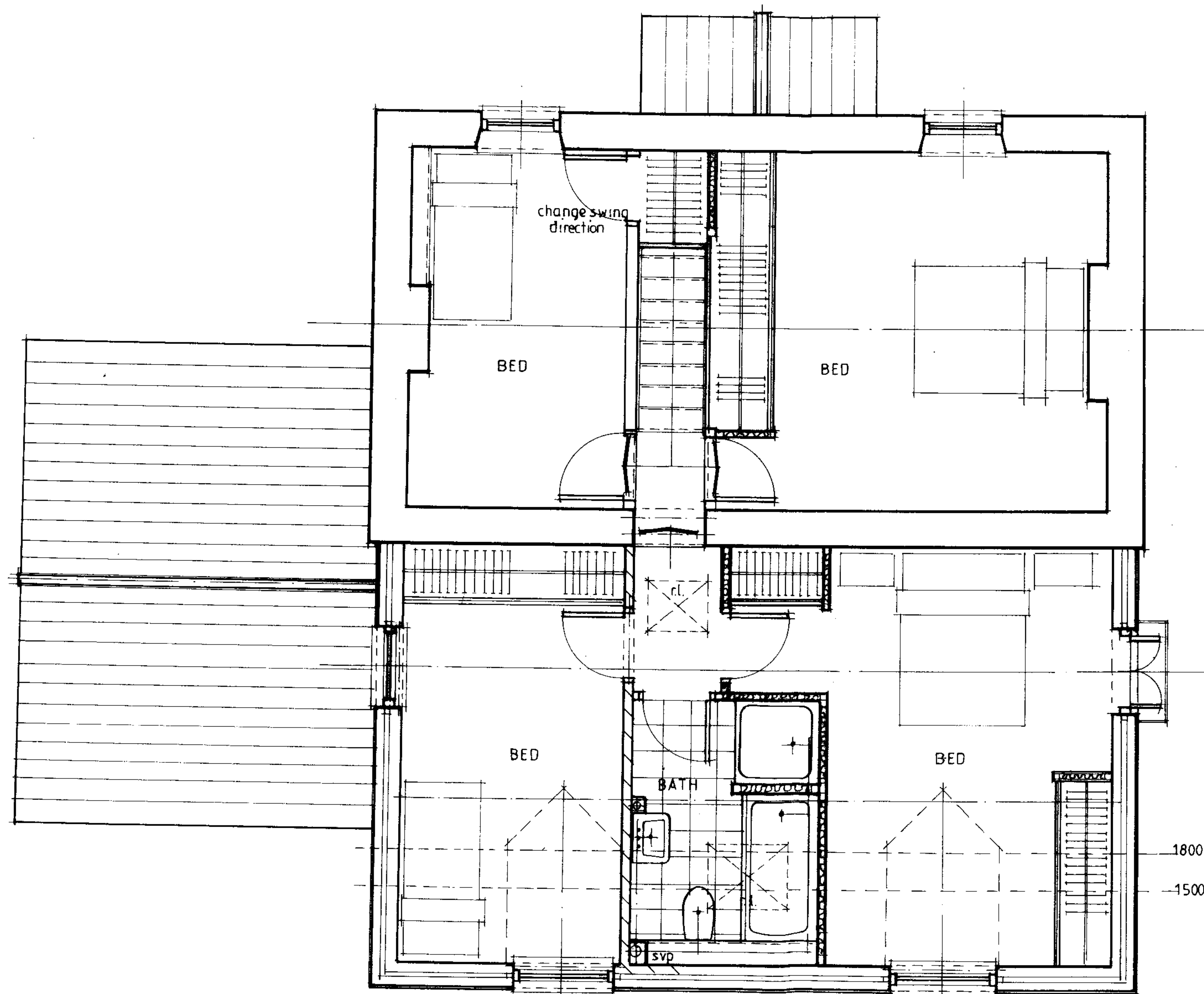
FIRST FLOOR PLAN 1: 50 (PROPOSED)
