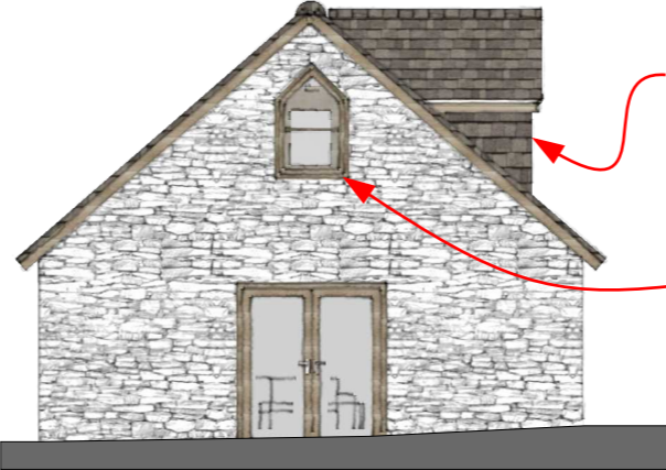
EAST ELEVATION 1:100
