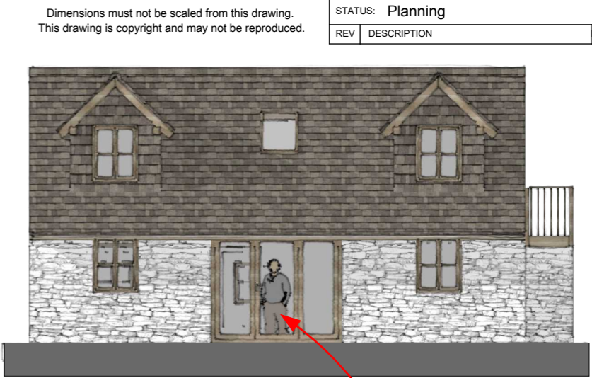
NORTH ELEVATION 1:100
