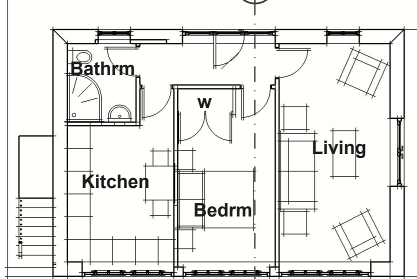
FIRST FLOOR 1:100
