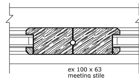
BI-FOLD MEETING STILE DETAIL - 1:5
