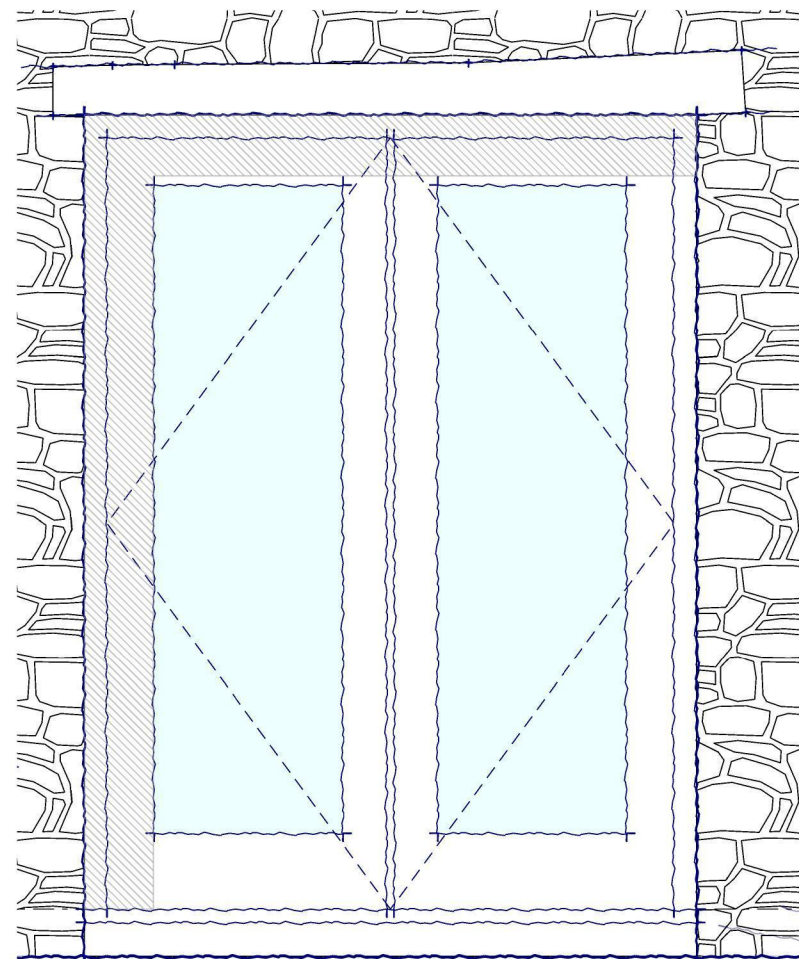
FRENCH CASEMENT ELEVATION - 1:10
