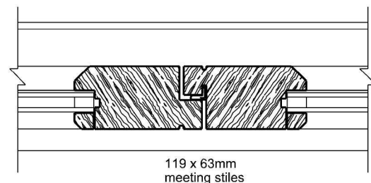
FRENCH CASEMENT MEETING STILE DETAIL - 1:5
