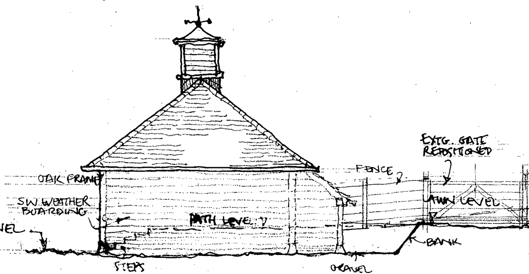
SOUTH ELEVATION
