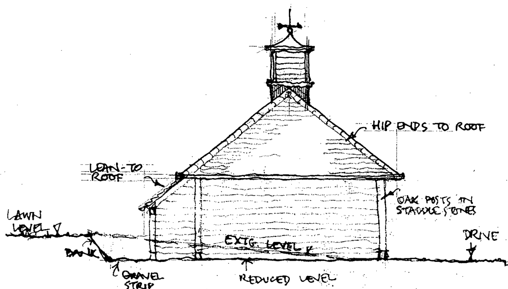
NORTH ELEVATION.
