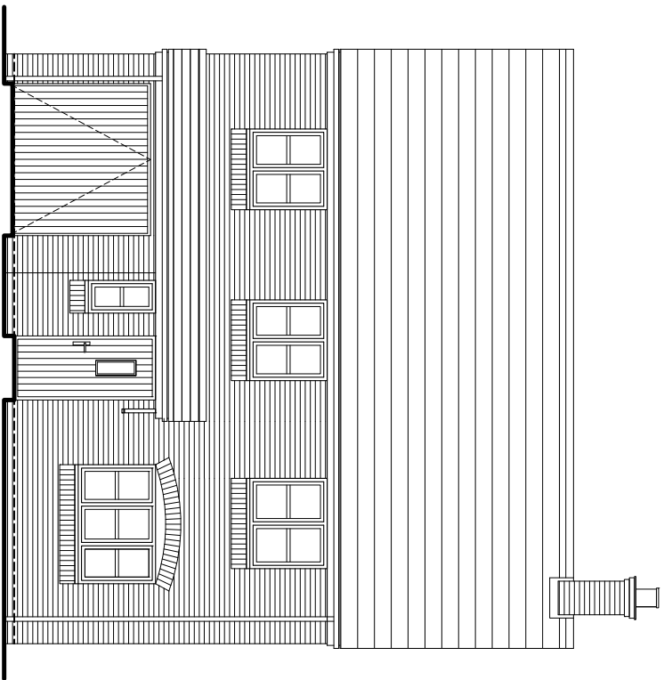
1570 OPTION 1 FRONT ELEVATION
