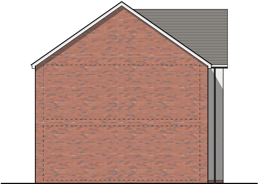
Gable Elevation Plot 21
