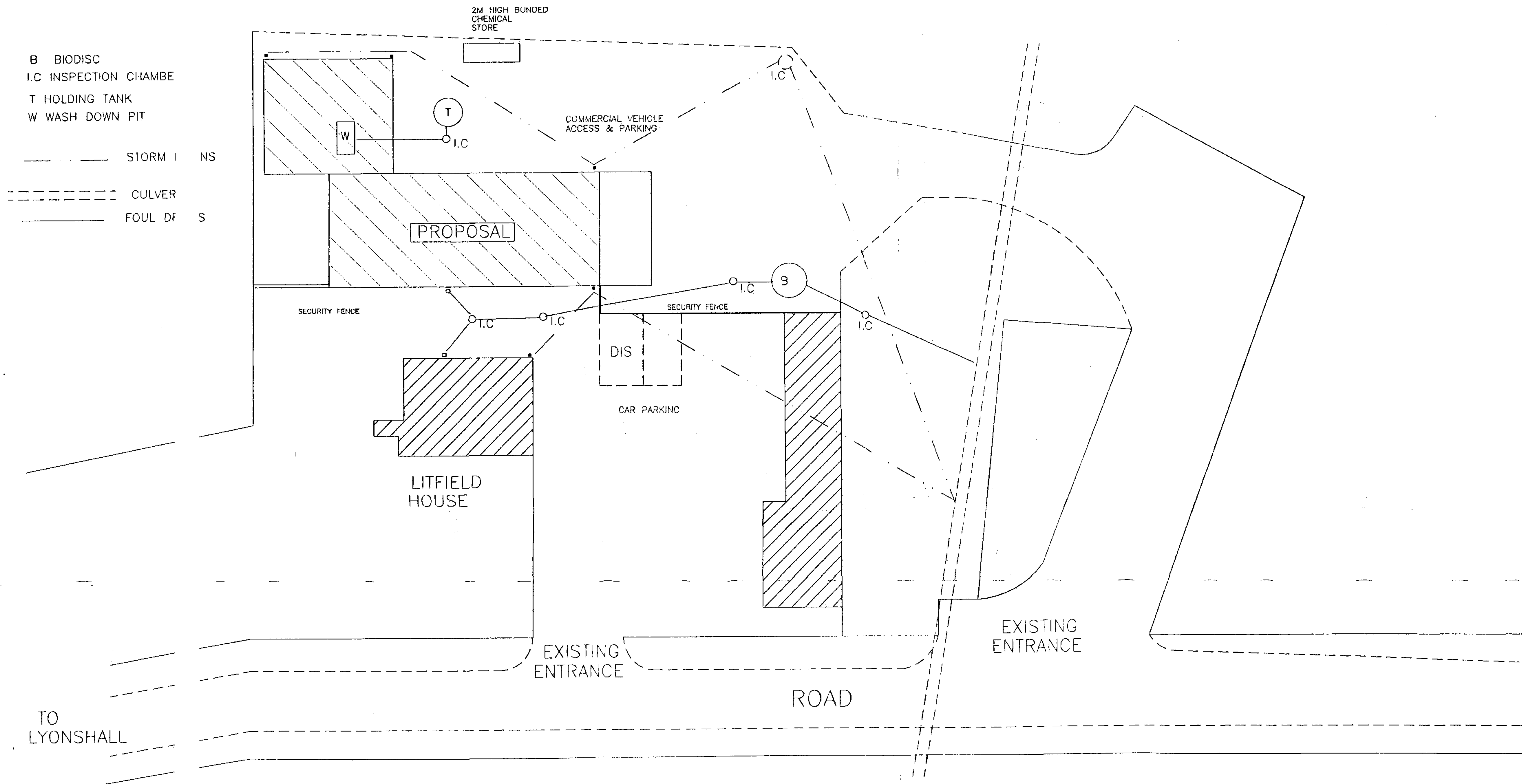
SITE PLAN SCALE 1:500
