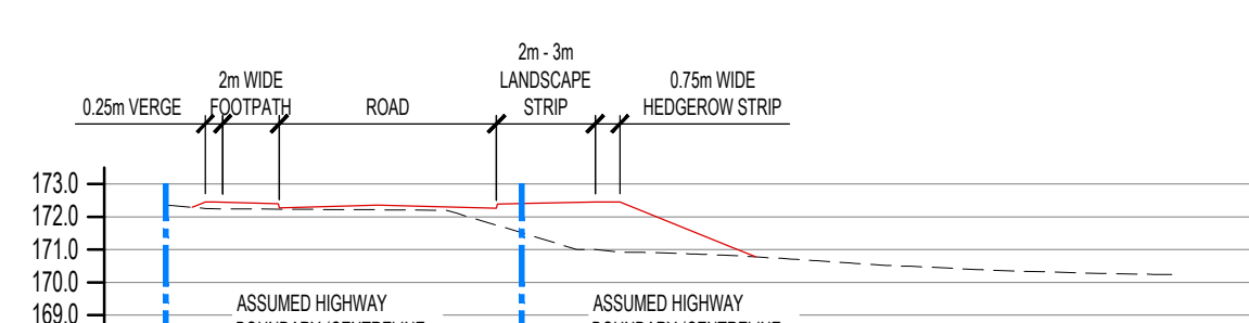
SECTION 15-15 (SCALE 1:250)
