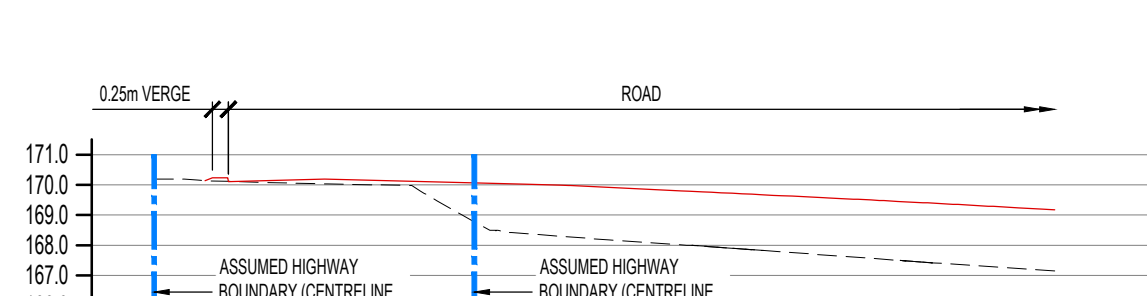
SECTION 8-8 (SCALE 1:250)
