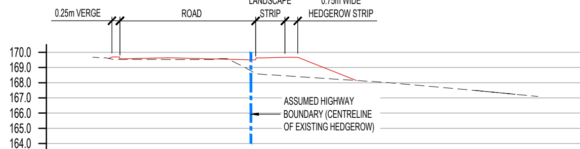
SECTION 6-6 (SCALE 1:250)
