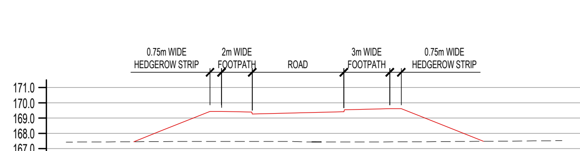
SECTION 20-20 (SCALE 1:250)
