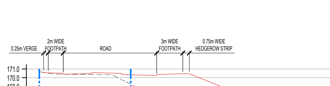
SECTION 10-10 (SCALE 1:250)
