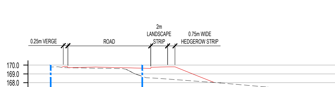
SECTION 5-5 (SCALE 1:250)
