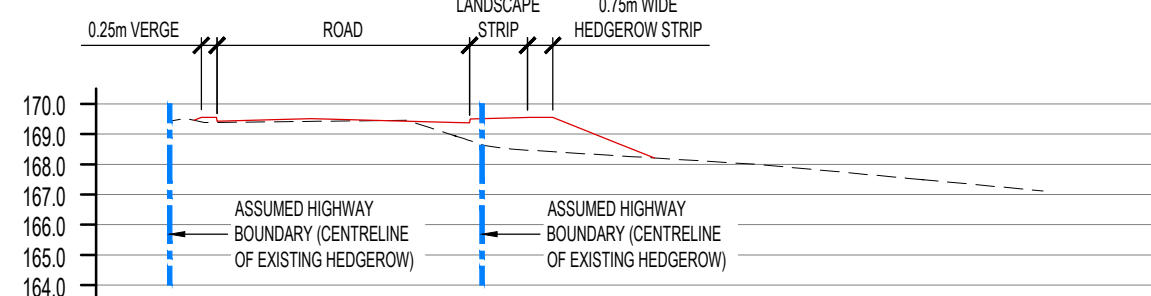
SECTION 5-5 (SCALE 1:250)
