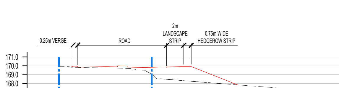
SECTION 6-6 (SCALE 1:250)
