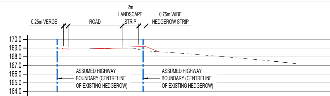
SECTION 1-1 (SCALE 1:250)
