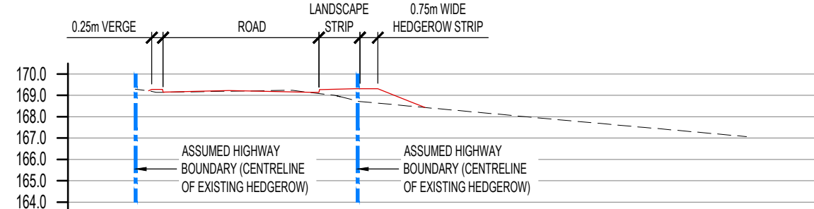
SECTION 3-3 (SCALE 1:250)
