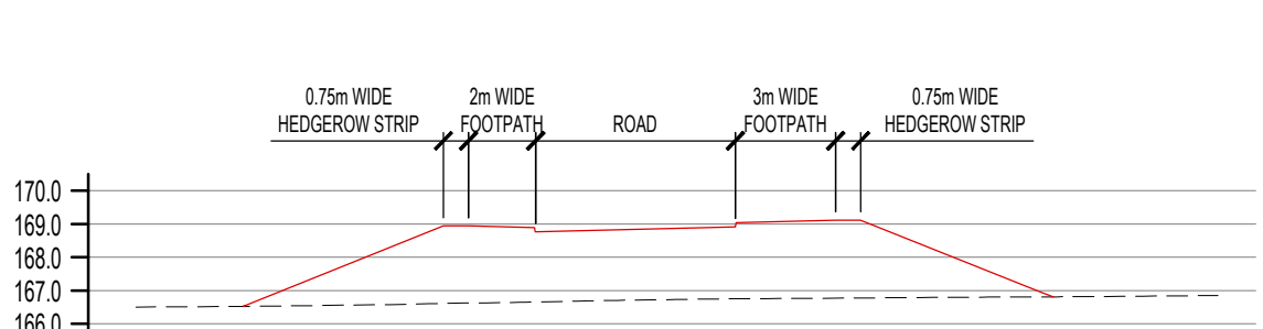
SECTION 21-21 (SCALE 1:250)
