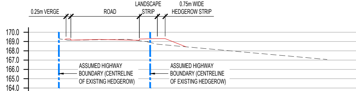
SECTION 4-4 (SCALE 1:250)
