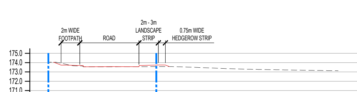
SECTION 19-19 (SCALE 1:250)
