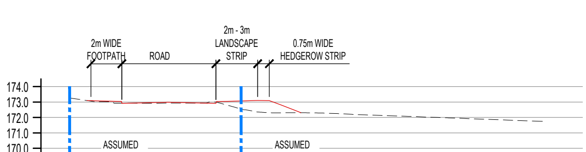
SECTION 17-17 (SCALE 1:250)
