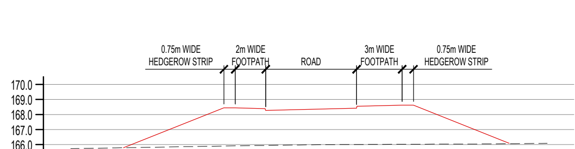
SECTION 22-22 (SCALE 1:250)
